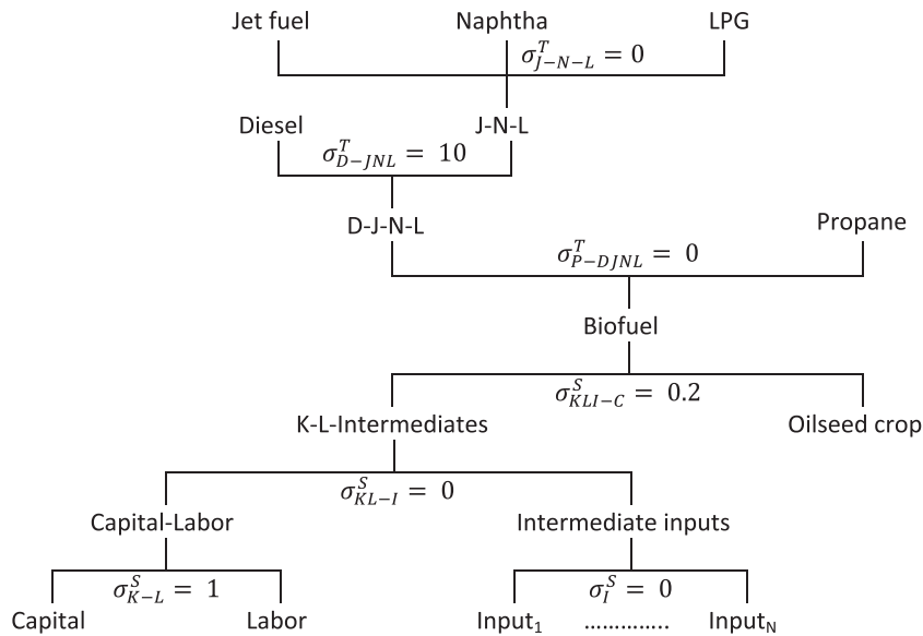
Fig. 1. Production of HEFA fuels in the EPPA-A model.
