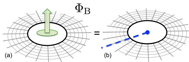
FIG. 11. (Color online) (a) Thread a gauge flux \Phi_B through a 1D ring (the boundary of 2D SPT). (b) The gauge flux is effectively captured by a branch cut (the dashed line in the blue color). Twisted boundary condition is applied on the branch cut. The (a) and (b) are equivalent in the sense that both cases capture the equivalent physical observables, such as the energy spectrum.
