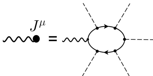
FIG. 7. In the fermionized language, one can capture the anomaly effect on induced (fractional) charge/current under soliton background by the one-loop diagram [43]. The solid line represents fermions, the wavy line represents the external (gauge) field coupling to the induced current J^\mu (or charge J^0 ), and the dashed line represents the scalar soliton (domain walls) background. Here in Sec. IV B, instead of fermionizing the theory, we directly address in the bosonized language to capture the bosonic anomaly.
