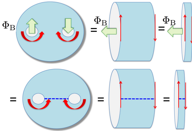
FIG. 2. (Color online) The intuitive way to view the bulk-boundary correspondence for edge modes of SPTs (or intrinsic topological order) under the flux insertion, or equivalently the monodromy defect/branch cut (blue dashed line) modifying the bulk and the edge Hamiltonians. SPTs located on a large sphere with two holes with flux-in and flux-out is analogous to a Laughlin-type flux insertion through a cylinder, inducing anomalous edge modes (red arrows) moving along the opposite directions on two edges.
