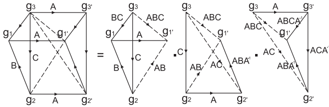
FIG. 9. The triangulation of a M^3 = M^2 \times I^1 topology (here M^2 is a spatial cylinder composed by the A and B directions, with a I^1 time) into three tetrahedra with branched structures.
