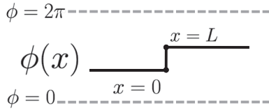
FIG. 4. We expect some fractional charge trapped near a single kink around x = 0 (i.e., x = 0 + \epsilon ) and x = L (i.e., x = 0 - \epsilon ) in the domain walls. For Z_{N_1} -symmetry-breaking domain wall with a kink jump \Delta\phi_1 = 2\pi \frac{n_{12}}{N_{12}} , we predict that the fractionalized (n_{12}/N_{12})p_{21} units of Z_{N_2} charge are induced.
