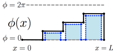
FIG. 6. (Color online) A profile of several domain walls, each with kinks and antikinks (in blue color). For Z_{N_1} -symmetry-breaking domain wall, each single kink can trap fractionalized Z_{N_2} charge. However, overall there is no nontrivial winding \int_0^L dx \partial_x \phi_1(x) = 0 (i.e., no net soliton insertion), so there is no net induced charge on the whole 1D ring.
