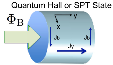
FIG. 13. (Color online) For topological phases, the anomalous current J_b of the boundary theory along the x direction leaks to J_y along the y direction in the extended bulk system. \Phi_B -flux insertion d\Phi_B/dt = -\oint E dL induces the electric E_x field along the x direction. The effective Hall effect dictates that J_y = \sigma_{xy} E_x = \sigma_{xy} \epsilon^{\mu\nu} \partial_\mu A_\nu , with the effective Hall conductance \sigma_{xy} probed by an external U(1) gauge field A .
