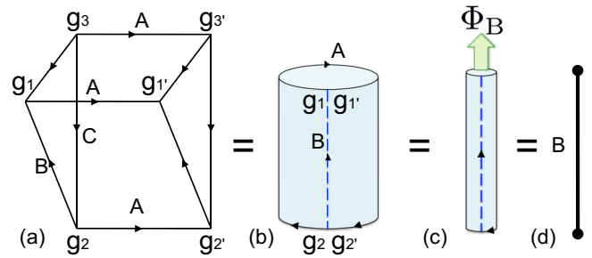
FIG. 8. (Color online) (a) The induced 2-cocycle from a 2+1D M^3 = M^2 \times I^1 topology with a symmetry-preserving Z_{N_u} flux A insertion. (b) Here M^2 = S^1 \times I^1 is a 2D spatial cylinder, composed by A and B , with another extra time dimension I^1 . Along the B line we insert a monodromy defect of Z_{N_1} , such that A has a nontrivial group element value A = g_1' g_1^{-1} = g_2' g_2^{-1} = g_3' g_3^{-1} \in Z_{N_1} . The induced 2-cocycle \beta_A(B, C) is a nontrivial element in \mathcal{H}^2(Z_{N_u} \times Z_{N_w}, U(1)) = \mathbb{Z}_{N_{vw}} (here u, v, w cyclic as e^{uvw} = 1 ), thus which carries a projective representation. (c) A monodromy defect can be viewed as a branch cut induced by a \Phi_B flux insertion (both modifying the Hamiltonians). (d) This means that when we do dimensional reduction on the compact ring S^1 and view the reduced system as a 1D line segment, there are N_{123} degenerate zero energy modes (due to the nontrivial projective representation).
