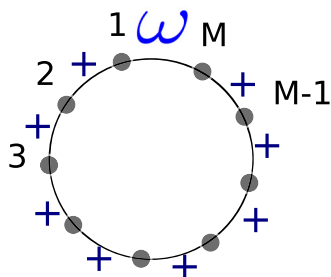
FIG. 12. (Color online) The illustration of an effective 1D lattice model with M sites on a compact ring under a discrete Z_N flux insertion. Effectively the gauge flux insertion is captured by a branch cut located between the site M and the site 1. This results in a Z_N variable \omega insertion as a twist effect modifying the lattice Hamiltonian around the site M and the site 1.
