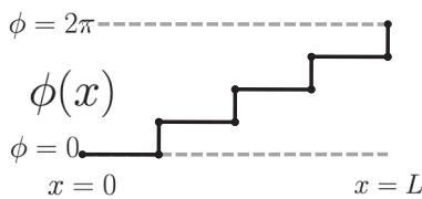
FIG. 5. A nontrivial winding \int_0^L dx \partial_x \phi(x) = 2\pi . This is like a soliton (or particle) insertion. For N_{12} number of Z_{N_1} -symmetry-breaking domain walls, we predict that the integer p_{21} units of total induced Z_{N_2} charge on a 1D ring. On average, each kink captures a p_{21}/N_{12} fractional units of Z_{N_2} charge.
