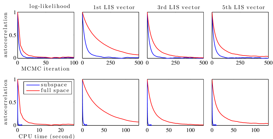
Figure 6. Autocorrelations of various benchmarks: blue line is subspace MCMC and red line is full-space MCMC. Column 1: log-likelihood function. Column 2: parameters projected onto the first LIS basis vector. Column 3: parameters projected onto the third LIS basis vector. Column 4: parameters projected onto the fifth LIS basis vector. Top row: Autocorrelation as a function of sample lag. Bottom row: Autocorrelation as a function of sample lag, where the latter is measured via CPU time.
