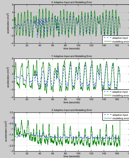
Fig. 3. The estimated modeling error is compared with the output of RBF adaptive element when using BKR-CL. It is seen that BKR-CL finds the correct weights and the RBF bases online required to learn the modeling uncertainty over time in x and y axes, however, the z axis performance suffers possibly due to unmodeled motor dynamics.
