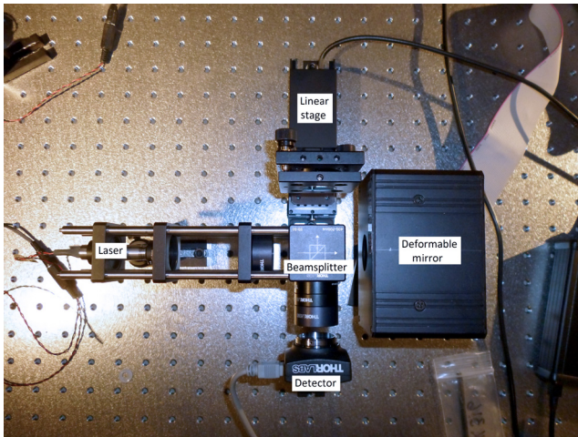
Fig. 4 CubeSat-sized MEMS DM Michelson interferometer prototype experiment. The setup includes a 1.5\ \mu\text{m} stroke Boston Micromachines Mini DM, a Thorlabs CPS180 635 nm 1 mW round beam collimated laser diode module, a cube beam splitter, a pinhole spatial filter, a neutral density filter, a flat mirror, and a Thorlabs DCC1545M \frac{1}{2} in. monochrome CMOS camera. A MATLAB interface to the mirror driver is commanding the 32 actuators into a “tilt” or “tip.”
