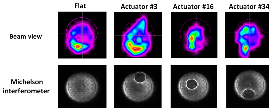
Fig. 7 Example results looking at different actuator “pokes” on the MEMS DM. The “beam view” is the laser intensity as reflected off of the MEMS DM.
