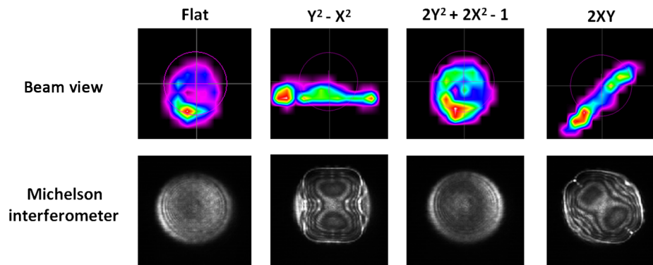
Fig. 8 Example results looking at different Zernike polynomials on the MEMS DM. The “beam view” is the laser intensity as reflected off of the MEMS DM.
