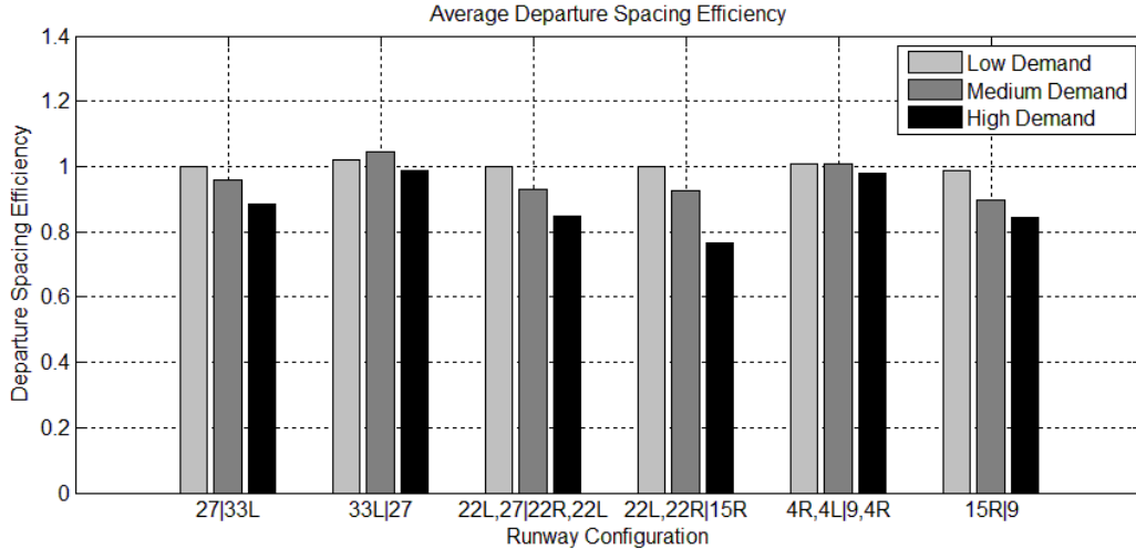
Figure 15: Average departure spacing efficiency for frequently used configurations at BOS.
