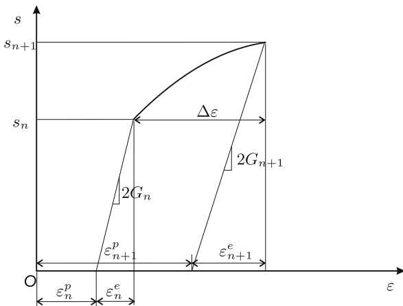
Fig. 15. A schematic drawing illustrates the evolution of the deviatoric stress tensor for the one-dimensional case.
