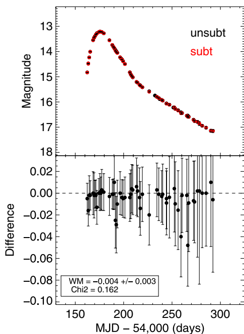
Figure 7. Comparison of the V-band unsubtracting and subtracting light curves of the bright SN 2007af. Most points agree to better than 0.01 mag. The weighted mean (WM) and \chi^2 of the differences are listed in the lower panel.
