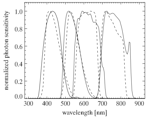
Figure 5. Synthesized natural system Keplercam BVr'i' passbands (solid curves) with Bessell (1990) BV and SDSS r'i' overplotted (dashed curves).
