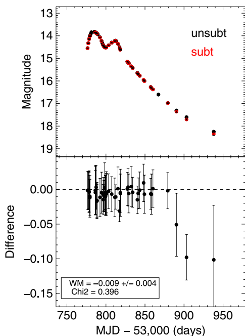
Figure 8. Comparison of the subtracting and unsubtracting i' light curves of the bright SN 2006X. Most points agree to better than 0.01 mag, suggesting that the reference-image subtraction is working well. The underlying galaxy flux only becomes evident at late times.
