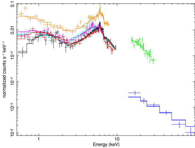
Figure 9. Counts spectra, best-fitting model, and residuals for all data. Shown are the Suzaku XIS FI (black), XIS BI (red), HXD PIN (green), Swift BAT (blue), Chandra Obs.ID 6910 (light blue), Chandra Obs.ID 7200 (magenta), and XMM-Newton pn (orange). The model fit shown is the sum of a partially covered power law, a soft, unabsorbed power law, and a Gaussian Fe K\alpha line (Model IV).
