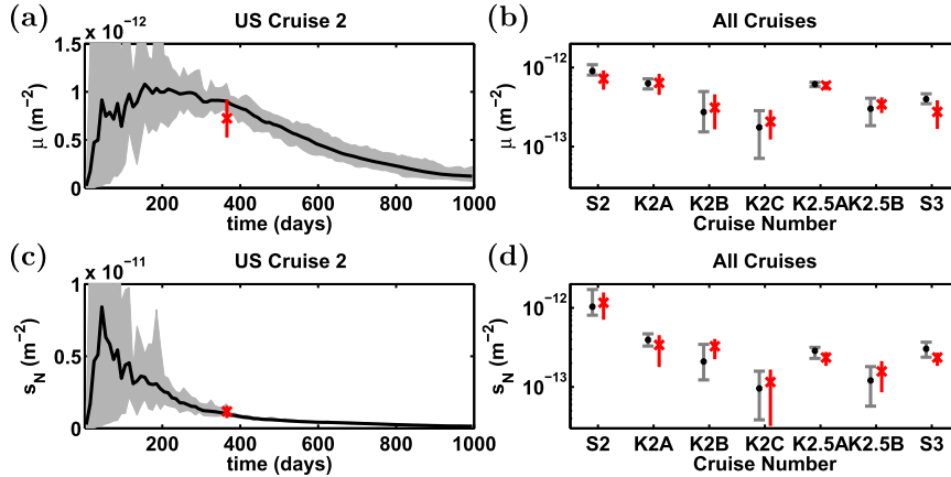
FIG. 6. (a) Modeled average ( \mu = N^{-1}\sum c_i ) and (c) standard deviation [ s_N = \sqrt{(N-1)^{-1}\sum (c_i - \mu)^2} ] of the column-integrated tracer concentration at the US2 cruise track locations vs time. The tracer concentrations are normalized by the total amount of tracer released; hence, the units are \text{m}^{-2} . The red x shows the observed tracer concentration from the DIMES US2 cruise, with the red line indicating a 95% confidence interval using bootstrapping. Gray shading indicates the minimum and maximum values from the 12 tracer releases from the ensemble. (b),(d) As in (a), but at the times listed in Table 1 for the four DIMES cruises. The UK2 and UK2.5 cruises have been split into individual transects from west to east (K2A, K2B, K2C, and K2.5A and K2.5B, respectively). US2 and US3 transects are represented by S2 and S3. Notice that we used a logarithmic scale in these two panels because the concentrations drop substantially 2 to 3 yr after injection.
