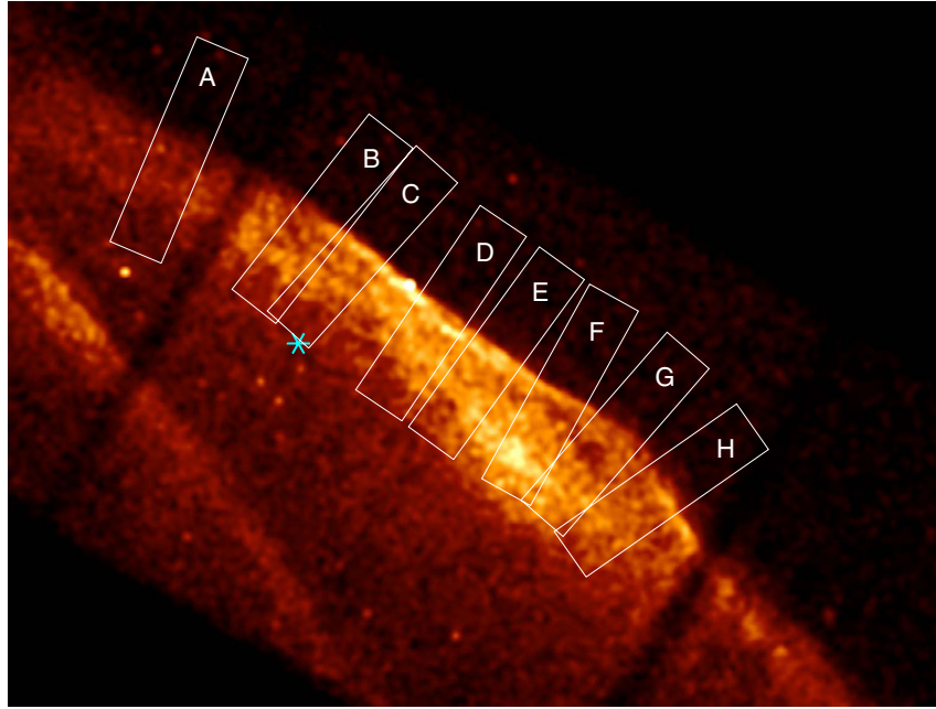
Figure 5. ACIS image of the northwestern rim of G266.2–1.2 for the same energy range shown in Figure 2. The bright filaments along the outer edge of the remnant are evident. The eight rectangles labeled A–H are the eight regions used to measure the widths of the bright X-ray-emitting filaments. The boxes are centered lengthwise on the portion of the rim with the largest surface brightness and are oriented at the angles that minimized the upstream filament widths l_1 . The asterisk marks the location of the optical axis of the telescope. See Section 3.1 and Table 4.
