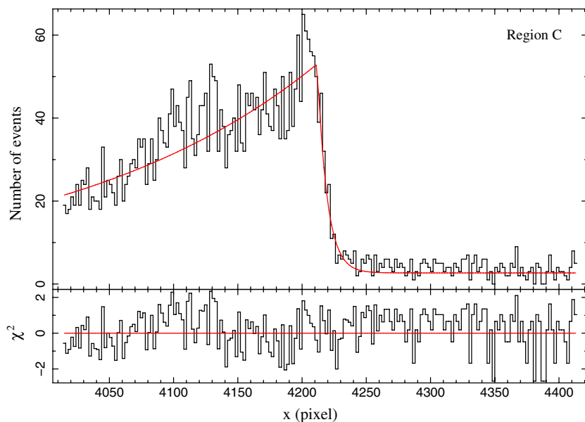
Figure 6. Histogram of the number of events in Region C as a function of the position x along the long axis of this region (top panel). The position angle of this axis is 312^\circ . The best-fit profile (see Equation (1)) is also shown in the top panel. The bottom panel shows the difference between the data and the model divided by the 1\sigma uncertainties in the data.
