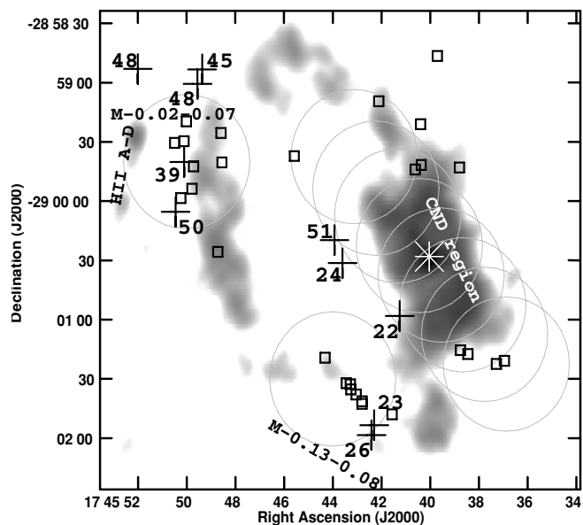
Figure 1. Gray scale outline of Sgr A in 1.7 GHz radio continuum with 1720 MHz OH masers (squares; see also Sjouwerman & Pihlström 2008). The newly detected 36 GHz methanol masers are located at the plus signs and labeled with their LSR velocities. The closest angular separation between any methanol and OH maser is 6'' (0.25 pc). Sgr A* is located in the dark CNDR region to the west (white star). The large gray circles show the 68'' diameter primary beams; the core of M–0.02–0.07 is covered by the easternmost beam.
