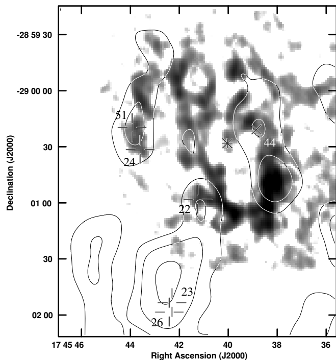
Figure 2. Integrated intensity contours of \text{NH}_3(3,3) emission and integrated intensity gray scale of \text{HCN}(4-3) emission outlining the ring-like CND (see also McGary et al. 2001; Montero-Castaño et al. 2009). The newly detected 36 GHz methanol masers near the CND (plus signs) are labeled with their LSR velocities, as is the 44 GHz methanol maser “V” (cross; Yusef-Zadeh et al. 2008). The star locates Sgr A* for reference. The \text{HCN}(4-3) image only partly covers the frame.
