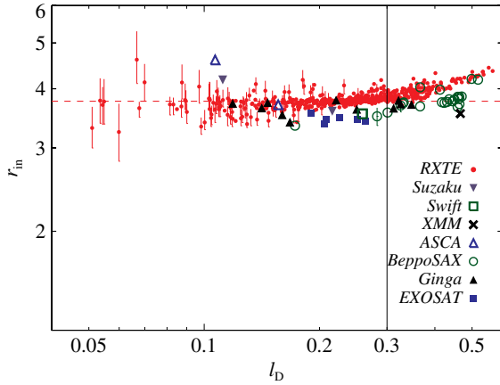
Figure 2. Dimensionless inner-disk radius r_{\text{in}} vs. luminosity for the filtered data (Section 3.1) and our baseline model. The vertical black line shows our adopted thin-disk upper limit, l_D = 0.3 . As in Figure 1, the red dashed line shows the RXTE average below this limit.
