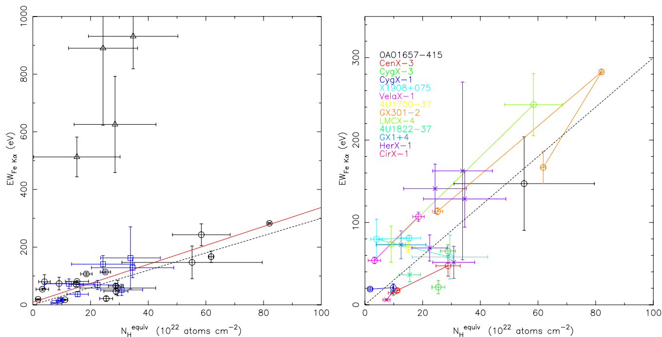
Figure 5. Left panel: the curve of growth. The EW of the Fe line grows with the column density of the reprocessing material (continuous red line) as predicted by the theoretical model of Kallman et al. (2004) for spherical geometry (dashed line). Black circles represent HMXB data and blue squares represent LMXB. Eclipse data (triangles, upper left corner) do not follow the main trend. Right panel: the several ObsIDs for the same source have been linked by a line, showing that, with few exceptions, the sources follow the relationship individually.
