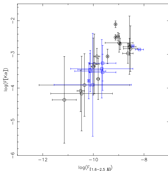
Figure 6. log–log plot of the line flux vs. the continuum flux. A good correlation exists ( F_{\text{line}} \propto F_{\text{cont}}^{0.71} ; r^2 = 0.75 ). The reprocessed fluorescence photons variations track closely the continuum emitted by the X-ray source. This means that the reprocessing region is very close to the X-ray continuum source. Black circles represent HMXB and blue squares LMXB.
