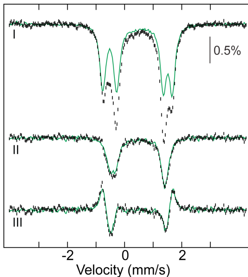
Figure 2. 4.2-K/53-mT Mössbauer spectra of the product of forward radical translocation trapped in the (Y_{731}NH_2Y-\alpha)_2\beta_2 complex. (I) Sample prepared with \beta , Y_{731}NH_2Y-\alpha , ATP and CDP. The green line is the scaled control spectrum of \beta that had been incubated with pathway-blocked Y_{731}F-\alpha , ATP and CDP, and subtraction of this spectral contribution reveals the spectrum of the product of forward radical translocation (II). The green line overlaid in II is the spectrum of the radical translocation product induced with N_3UDP from Fig.1B, III, and is shown to illustrate the near identity of the perturbed spectra resolved by the two different trapping approaches. The spectrum in III is the total difference of the spectrum of (Y_{731}F-\alpha)_2\beta_2 in the presence of ATP and CDP subtracted from I, and the green line is the total difference spectrum from the \alpha_2\beta_2 \pm N_3UDP experiment in Fig.1B, IV.
