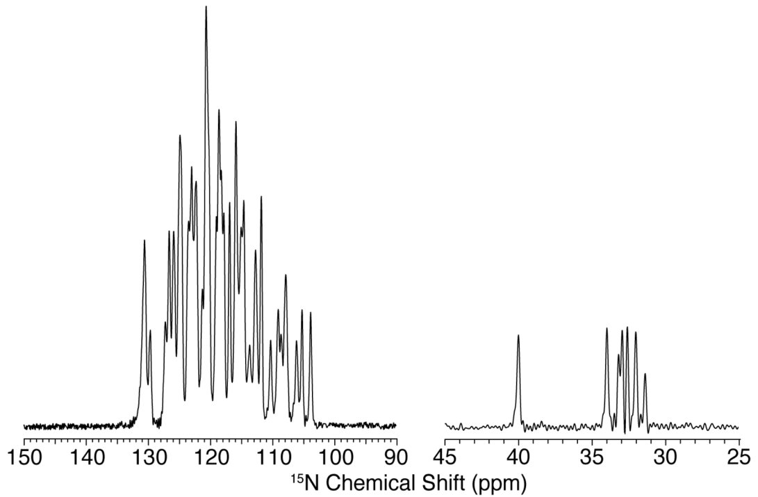
Figure 3. ^{15}\text{N} CP MAS spectrum of [ \text{U-}^{15}\text{N} , redox- ^{13}\text{C} ] labeled microcrystalline GB1. The spectrum was obtained at 800 MHz ^1\text{H} Larmor frequency with 18.0 kHz MAS and 81 kHz TPPM ^1\text{H} decoupling; 1024 points were acquired with a 50 \mu\text{s} dwell time for a total acquisition time of ~51 ms.
