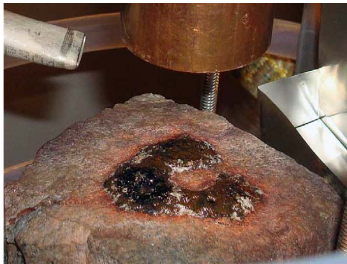
Figure 6. Granite rock surface 52 mm distant from waveguide aperture showing TE_{01} pattern.
