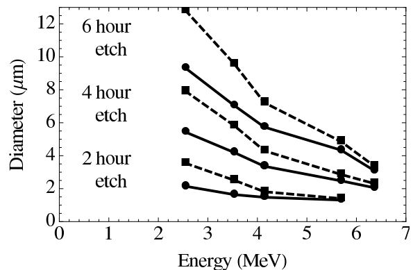
FIG. 7. Diameter of tracks observed versus energy for 2, 4, and 6 hours etch time. Solid lines represent the front CR-39 surface, dashed lines represent the back surface. Example distributions are shown in Fig. 6
