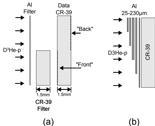
FIG. 4. Filtering configuration for the accelerator fusion product source experiments. Fig. (a) shows that filters for equivalent known energy distributions at the front and back surface of a single detector using both Al and a CR-39 filter. Fig. (b) shows that several energy windows are created through different Al thicknesses. Figs (a) and (b) are orthogonal depictions of the filter pack. For a given Al thickness, a CR-39 filter is used to create identical energy distributions at the front and back surface of the data CR-39 (a). In an orthogonal direction, multiple Al thicknesses are used to vary the energy distribution over five windows (b).
