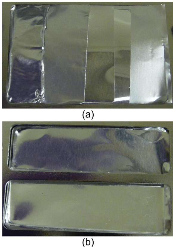
FIG. 5. Images of the filter pack used in this experiment. (a) Front view (looking along proton trajectory) of filter pack. Five energy windows are created via varying the aluminum thickness, which increases from right to left. (b) Back view (looking towards proton source) of filter pack. The CR-39 filter is visible in the bottom half.
