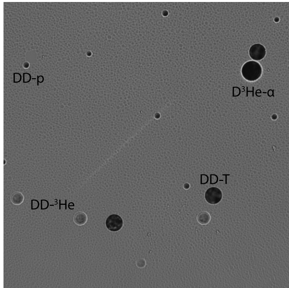
FIG. 2. Four types of particle track in CR-39 after a 3 hour etch. Shown are DD-p ( D \approx 4\mu\text{m} ), DD- {}^3\text{He} ( D \approx 9\mu\text{m} ), DD-T ( D \approx 13\mu\text{m} ), and D^3\text{He}-{}^4\text{He} ( D \approx 14\mu\text{m} ). For DD-p, DD-T, and D^3\text{He}-{}^4\text{He} the track contrast is \geq 90\% as defined in this work; the DD- {}^3\text{He} have contrast 60 – 70% (see Appendix B). The 14.7 MeV D^3\text{He} protons are undetectable in this scheme, since they are not ranged down into the detectable energy range. The CR-39 was filtered with only 1\mu\text{m} of aluminized mylar to allow detection of the {}^3\text{He} ions. The image size is 208\mu\text{m} square.
