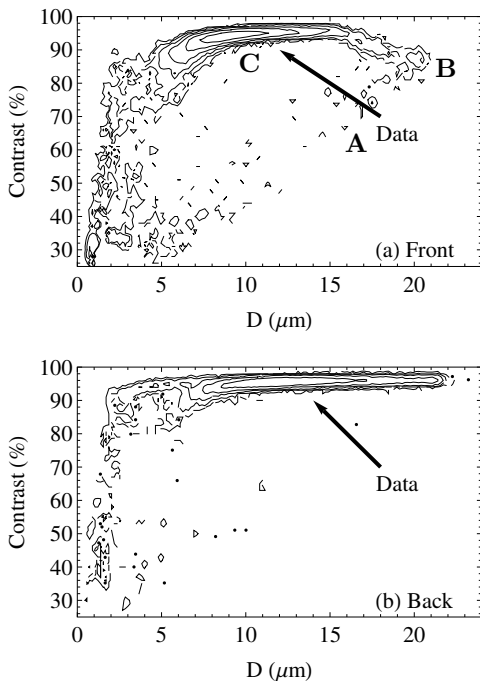
FIG. 8. Contour plots of the number of tracks versus track contrast and diameter for the same piece of CR-39 in Fig. 6. Data for 2.55 MeV protons is shown for the front side (top, with regions of data identified with stopping power regimes) and the back side (bottom). Intrinsic CR-39 noise appears in the low-contrast low-diameter regime. Contours represent a constant number of tracks per unit contrast and diameter; the values of this quantity corresponding to plotted contours form a geometric series with a ratio of 3. As defined in this work a high contrast number is a dark track, while a low contrast number is a light track (see Fig. 2).
