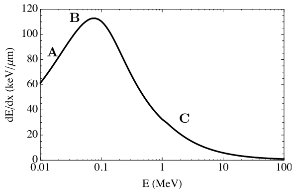
FIG. 9. Stopping power for protons in CR-39, given as change in energy per unit length. Protons of order MeV (C) create small dark tracks. Around the Bragg peak (B) protons create large tracks due to the large dE/dx . For protons that stop in the etched plastic (A) the track etches away and becomes light and hard to detect. These features are labeled in Fig. 8(a)
