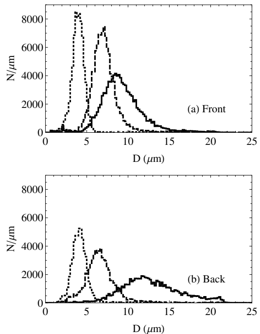
FIG. 6. Sample track diameter spectra on a single CR-39 detector for the front (a) and back (b) sides of the CR-39 SSNTD after 6 hours etching time. The incident energy distributions observed are identical in each case (see Fig. 4) with mean energies of 2.55 MeV (solid line), 4.14 MeV (dashed line), and 5.68 MeV (dotted line). Contrast plots for the 2.55 MeV data are shown in Fig. 8.
