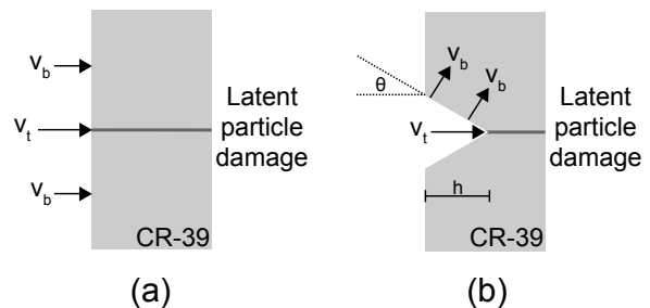
FIG. 3. An overview of the track etching process in SSNTDs. Fig. (a) shows the SSNTD at the start of the etch process. The latent particle damage is unobservable with conventional techniques ( \sim 5\text{ nm} in size). Fig. (b) shows that after some etch time a track is developed. Typical track diameters are 2– 30\mu\text{m} depending on particle species, energy, and etch time.
