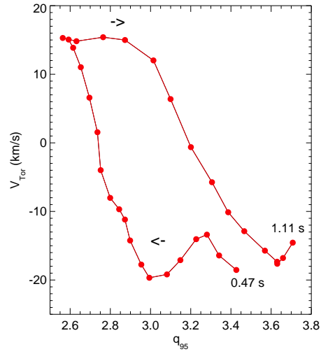
Figure 7: The discharge trajectory in the q_{95} - V_{Tor} plane for the plasma shown by the solid lines in Fig.6. Points are separated by 20 ms. Arrows indicate temporal direction.
