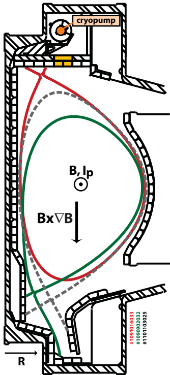
Figure 2. Typical shape of C-Mod last closed flux surface for I-mode experiments in unfavorable drift (red, upper x-point) and favorable drift (green, lower x-point). Plasmas in more usual C-mod configurations (e.g. dashed grey curve) have not exhibited transitions to I-mode.
