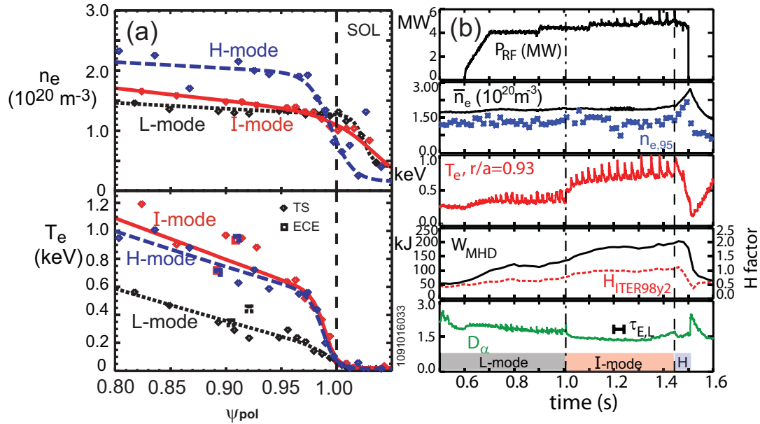
Figure 1: (a) Edge profiles of electron density (top) and temperature (bottom) for different phases of a 1.2 MA, 5.6 T C-Mod discharge (1091016033). Curves have been fit using a modified tanh function as described in Ref 28. The I-mode phase (red solid line, 1.41 s) has a steep T_e gradient, but a density profile close to that in L-mode (black dotted line, 0.78 sec). In a brief ELM-free H-mode (blue dashed curve, 1.47 s) T_e is similar to I-mode but n_e is much steeper). (b) Time histories of input ICRF power (top) and plasma parameters for the same discharge. In fourth panel, solid black curve is stored energy, and dashed red curve is confinement normalized to IPB98y2 scaling, reaching 1 in I-mode [18].
