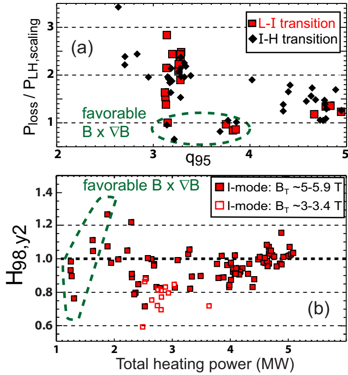
Figure 4. (a) Power thresholds for the L-I transition (red squares) and I-H transition (black diamonds), normalized to the Martin scaling [17]. The circled points are for favorable configuration and fit the scaling, while the remaining points, in unfavorable drift, are significantly higher. (b) Energy confinement time for I-mode discharges, normalized to the IPB98y2 scaling [18]. Average H_{98} is about 1, in both configurations, for discharges with B_T > 5 T (closed symbols) and about 0.8 for B < 3.5 T (open symbols).
