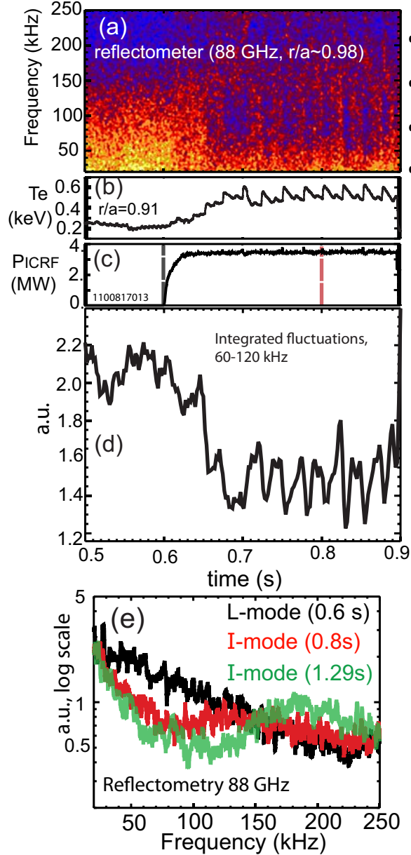
Figure 6. Evolution of fluctuations and edge T_e for a q_{95}=3.8 C-Mod discharge 1100817013 (1.1 MA, 5.6 T, upper single null). (a) Contours of reflectometer fluctuations (88 GHz, n_c = 9.6 \times 10^{19} \text{ m}^{-3} ( r/a \approx 0.98 )). (b) T_e at r/a \approx 0.91 , showing a gradual increase after application of ICRF power (c). (d) Integrated reflectometry fluctuations in the band 60-120 kHz, which are anticorrelated with T_e both during the L-I transition period and at sawtooth heat pulses in the steady I-mode phase. (e) Reflectometry spectra in the L-mode (black) and I-mode (red) phases indicated by bars in (c), and during a later I-mode phase with slightly higher T_e (green).
