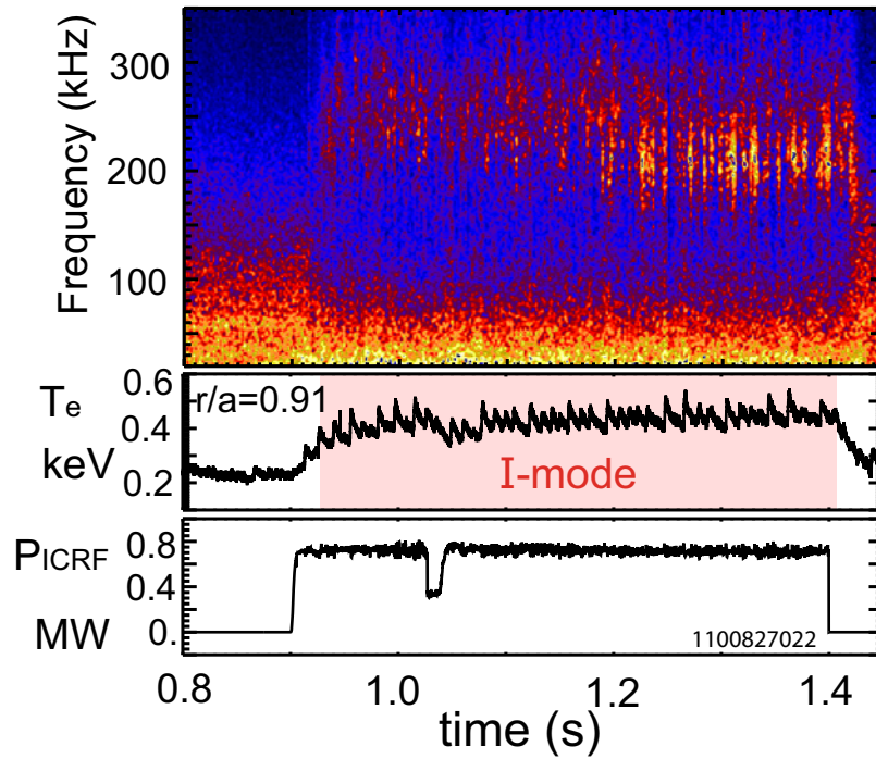
Figure 3. Steady I-mode achieved in favorable configuration (C-Mod discharge 1100827022, 0.8 MA, 5.4 T, lower single null). Density fluctuations measured by o-mode reflectometry (top panel), at n_c=7 \times 10^{19} \text{ m}^{-3} ( r/a \cong 0.98 ), show a decrease in mid-f turbulence and the appearance of a broad high f feature soon after the application of 0.75 MW ICRH (bottom). The I-mode phase, which has edge T_e significantly above that in similar L-mode discharges (middle panel) lasts for the duration of the RF pulse, about 10 \tau_E .
