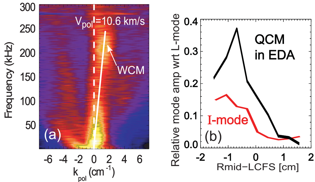
Figure 9. (a) Emission fluctuations measured by Gas Puff Imaging at the horizontal midplane during an I-mode phase of C-Mod discharge 1100204022 (1.3 MA, 5.8 T, upper single null). A Weakly Coherent Mode is visible, centered at about f=220 kHz, k_{pol}=+1.25 \text{cm}^{-1} (electron diamagnetic direction). (b) Relative amplitude of the WCM (increase over L-Mode turbulence, normalized to average intensity) vs. radius (red). The radial profile of the Quasicoherent Mode in an EDA H-mode is shown for comparison (black).
