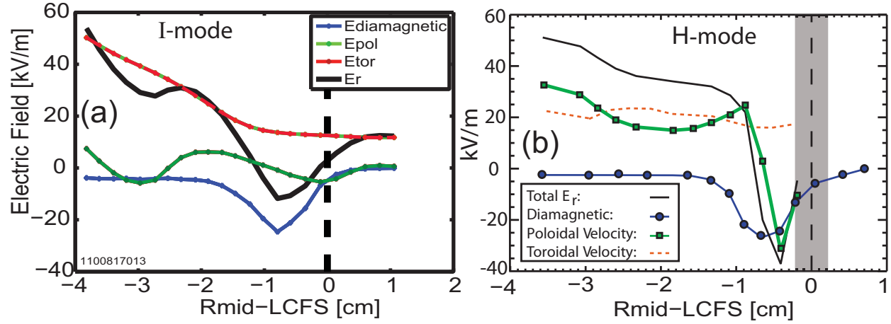
Figure 8. (a) Radial electric field in a 1.1 MA I-mode discharge, derived from the CXRS profiles shown in Fig. 7. The 30 keV/m well in total E_r (black) is dominated by the diamagnetic term (blue), with a significant gradient from the V_{\text{tor}} \times B_{\text{pol}} term (red). (b) For comparison, an E_r profile in a typical EDA H-mode, with I_p=800 kA, which has a stronger contribution from the V_{\text{pol}} \times B_{\text{tor}} term (green). From R. McDermott et al, Phys. Plasmas 16 , 056103 (2009).
