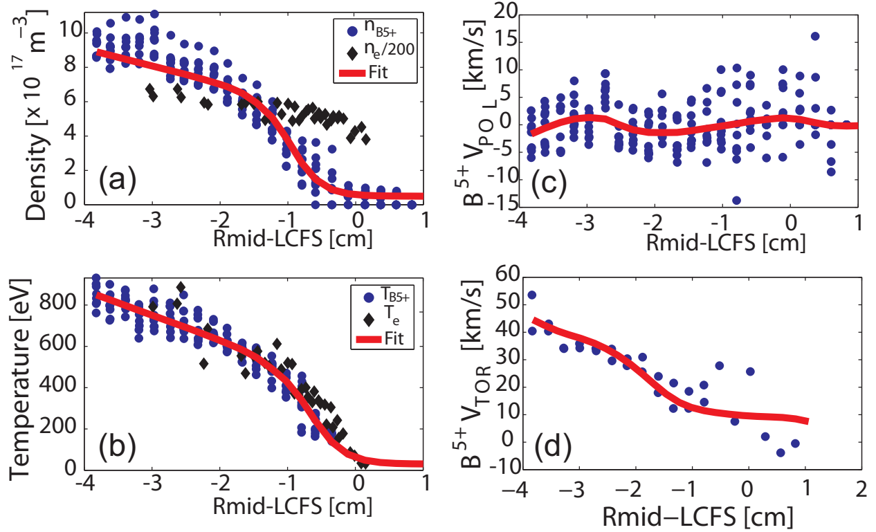
Figure 7. CXRS profiles for boron +5, averaged over I-mode phases of the same discharge as in Fig. 6. Note that n_{B^{5+}} (a) does not have the same profile as n_e (black diamonds, scaled by 200 for comparison). Its temperature pedestal (b), however, is the same as T_e measured by edge TS (black diamonds) within respective mapping uncertainties. V_{pol} (c) is flat and near zero, while V_{tor} (d) exhibits co-current rotation of up to 40 km/s.
