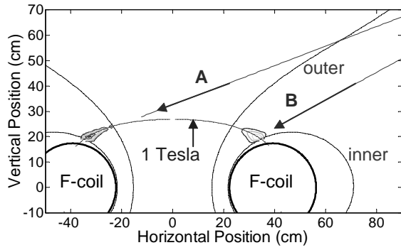
Figure 1. Cross section of LDX F-coil and flux surfaces showing 10 keV EC absorption coefficient contours for 28 GHz incident rays A and B
