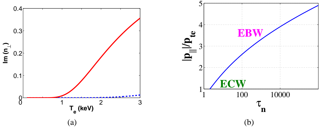
Figure 2: (a) Im(n_{\perp}) versus electron temperature for NSTX-type plasmas with \omega/\omega_{ce} = 1.9 , \omega_{pe}/\omega_{ce} = 6 , and n_{\parallel} = 0.2 ; (b) The parallel electron momentum normalized to the thermal momentum versus the optical depth for the electron cyclotron waves. ECW represents the X and O waves.
