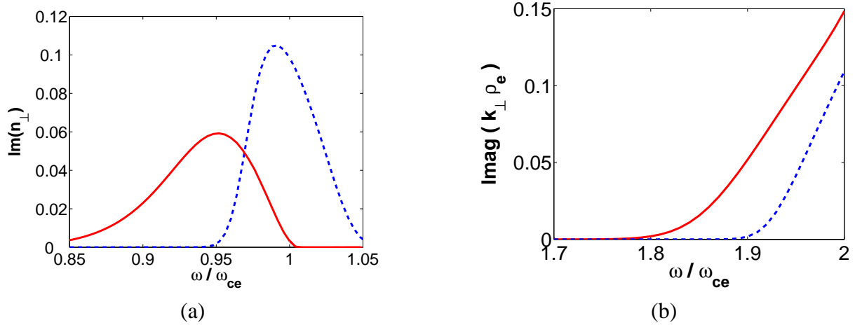
Figure 1: (a) Imaginary- n_{\perp} for an O wave versus \omega/\omega_{ce} for ITER-type parameters with \omega/2\pi = 170 GHz, electron temperature T_e = 10 keV, \omega_{pe}/\omega = 0.75 ( \omega_{pe} is the electron plasma frequency), and n_{\parallel} = 0.1 ; (b) imaginary part of (k_{\perp}\rho_e) for an EBW versus \omega/\omega_{ce} for NSTX-type parameters with \omega_{pe}/\omega_{ce} = 6 , T_e = 3 keV, and n_{\parallel} = 0.2 .
