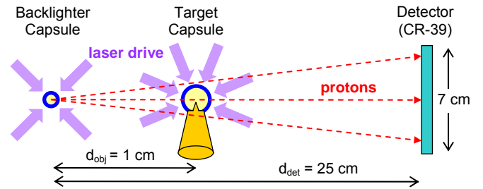
Fig. 1: Schematic of the experimental setup. A short (130 ps), monoenergetic ( \Delta E/E < 3\% ), quasi-isotropic pulse of 15.0-MeV \text{D}^3\text{He} fusion protons is generated by laser implosion of a backlighter capsule filled with \text{D}_2 and ^3\text{He} gas. The \sim 3 \times 10^8 protons emitted from the 45- \mu\text{m} full width at half maximum source region interact with matter and electromagnetic fields in a cone-in-shell capsule implosion. The position and energy of every proton reaching the detector are individually recorded on CR-39, encoding the details of the matter and field distributions surrounding the target capsule.
