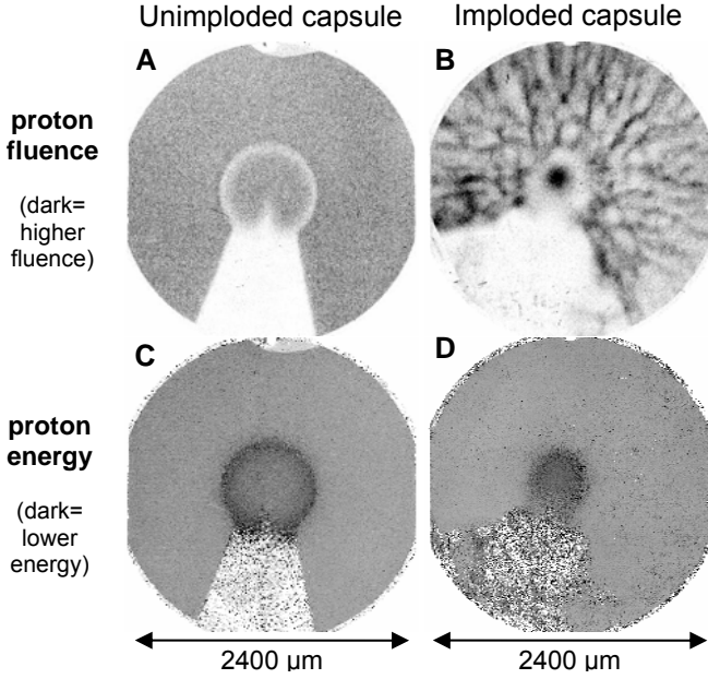
Fig. 3: Images of a 430- \mu\text{m} -radius spherical plastic capsule with attached Au cone, before and during implosion. (A and C) Unimploded capsule used in OMEGA shot 46531. (B and D) Capsule at 1.56 ns after the onset of the laser drive (OMEGA shot 46529). The dark areas correspond to regions of higher proton fluence [in (A) and (B)] and regions of lower proton energy [in (C) and (D)]. The energy image values in the region shadowed by the cone are mostly noise because very few protons were detected in that region. See lineouts in Fig. 4 and 5 for image values.
