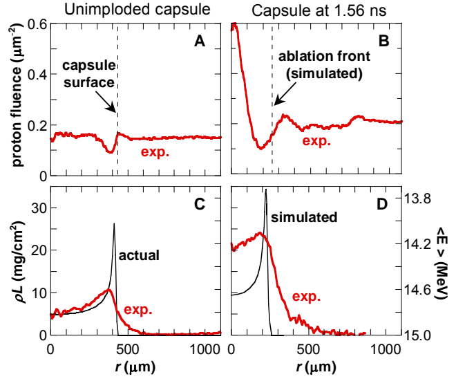
Fig. 4: Experimental (exp) radial lineouts (red lines) of proton fluence and mean path areal density ( \rho L ) from Fig. 3. All lineouts are averaged over the azimuth, excluding the region of the cone shadow. (A and C) Unimploded capsule of OMEGA shot 46531. (B and D) Capsule of OMEGA shot 46529, 1.56 ns after start of laser drive. The fluence lineout (A) shows the effects of angular scattering through the limb of the capsule shell. In (B), angular scattering effects alone are insufficient to explain the peak at r = 0 . A radial electric field of \sim 10^9 V/m is necessary to focus the protons to the extent observed. In (C) and (D), radial lineouts of the mean energy images in Fig. 3 were converted to \rho L . Also displayed are the actual \rho L (C) and simulated \rho L (D), assuming no angular scattering (black line). \rho R is given by \rho L/2 at r = 0 .
