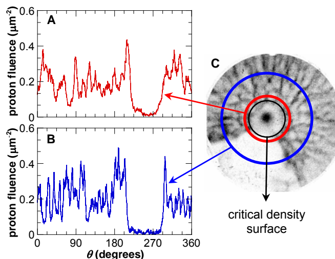
Fig. 5: Circular lineouts of proton fluence obtained from OMEGA shot 46529 at radii of 430 \mu\text{m} (A) and 860 \mu\text{m} (B). The filamentary structures represent a 2-dimensional (2-D) projection of a 3-D field structure that originates inside the critical density surface (C).
