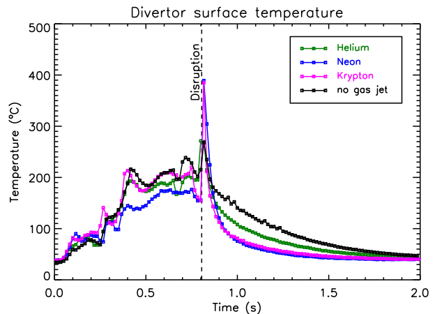
Figure 4. IR-derived temperature of the divertor surface during several different gas jet disruptions in C-Mod. Gas jet injection reduces the surface temperature compared to unmitigated disruptions. Higher Z gases do better than low Z .
