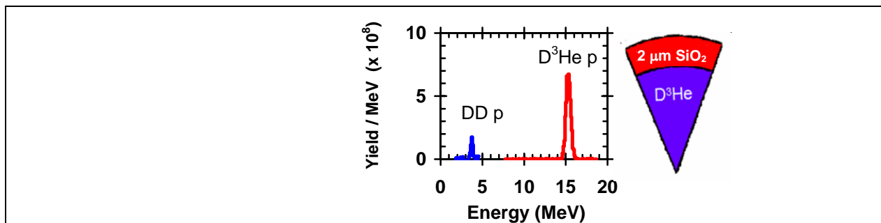
FIG. 1. Measured energy spectra of monoenergetic D^3He and DD protons generated in an implosion of a thin-glass shell filled with D^3He gas (OMEGA shot 42767). The data described in this Letter correspond to the D^3He protons; use of the 3-MeV DD protons will be explored in future work.
