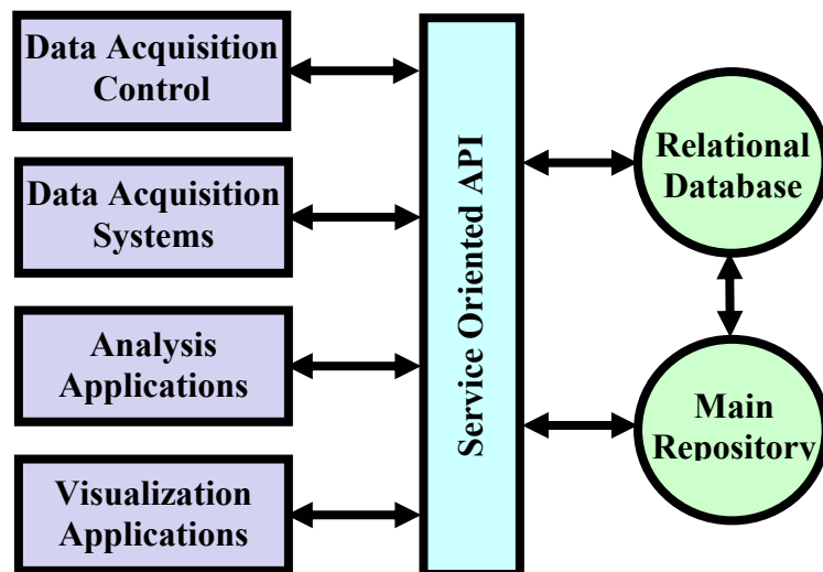
Figure 1. The proposed data system architecture would be comprised of two data structures: the main repository containing all the large multi-dimensional arrays and a queryable database containing all metadata, ancillary and high-level physics data. User interactions would be service-oriented; access would be through a single, simple, standard API and all applications would be data-driven.
