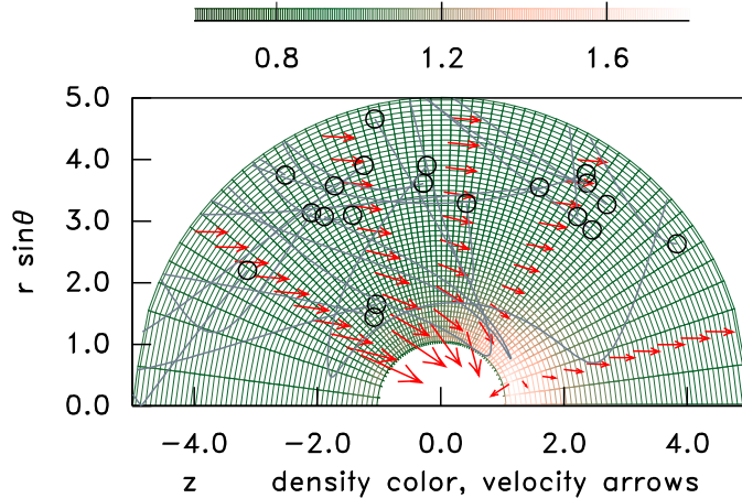
Figure 1: Computational grid of SCEPTIC. Color contours indicate the ion density, normalized to the value at infinity. Density is enhanced immediately downstream from the probe. Arrows show the mean (fluid) velocity, normalized to \sqrt{ZT_e/m_i} . The external flow (left to right) for this case is unity. The tracks of 20 (out of \sim 7M ) particle orbits are shown.
