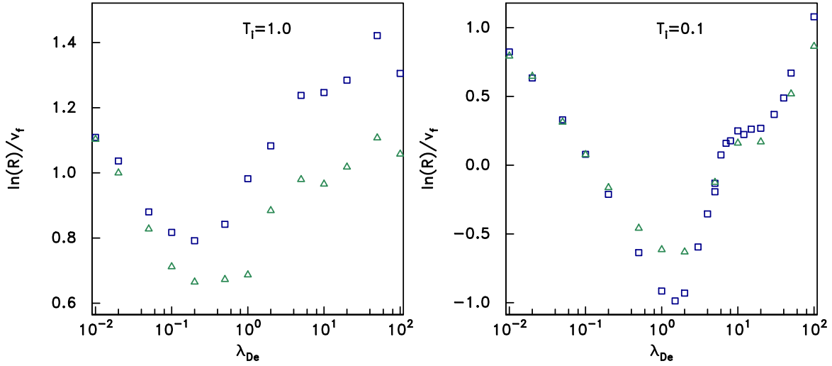
Figure 7: Asymmetry factor \ln(R)/v_f as a function of Debye length normalized to sphere radius. Squares: floating; triangles: insulating sphere.
