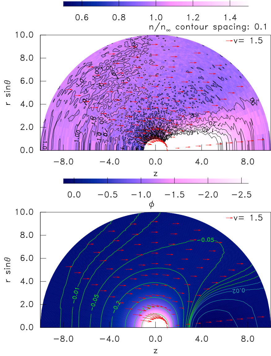
Figure 3: Contour plots of density (upper) and potential (lower) for a floating sphere when T_i = 0.1T_e , v_f = 1.5\sqrt{ZT_e/m_i} , \lambda_{De} = 2r_p , m_i = 1837m_e . The arrows show mean ion velocity. The potential contours are logarithmically spaced.
