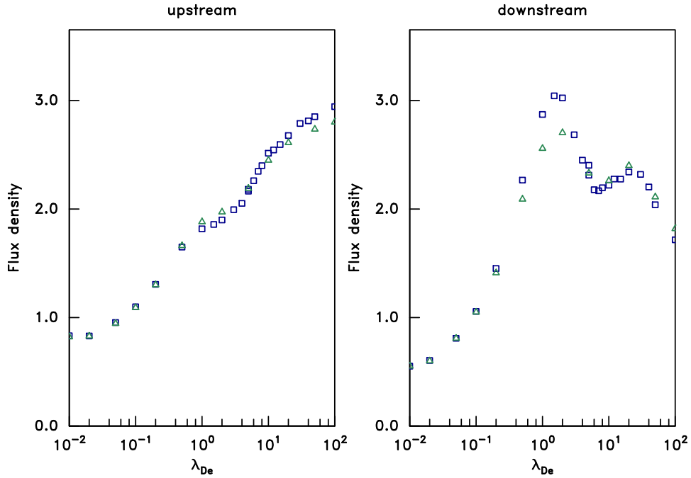
Figure 8: Flux density (in units of n_{i\infty} \sqrt{ZT_e/m_i} ) on the upstream and downstream axial positions as a function of Debye length (in units of r_p ), for drift velocity v_f = 0.5 (times \sqrt{ZT_e/m_i} ). Squares: floating; triangles: insulating sphere.
