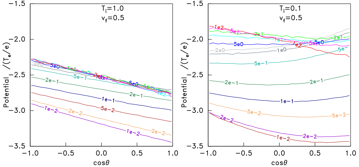
Figure 6: Surface potential as a function of angle for an insulating sphere for various values of \lambda_{De} normalized to the the sphere radius, fixed flow velocity, m_i/m_e = 1837 (hydrogen).
