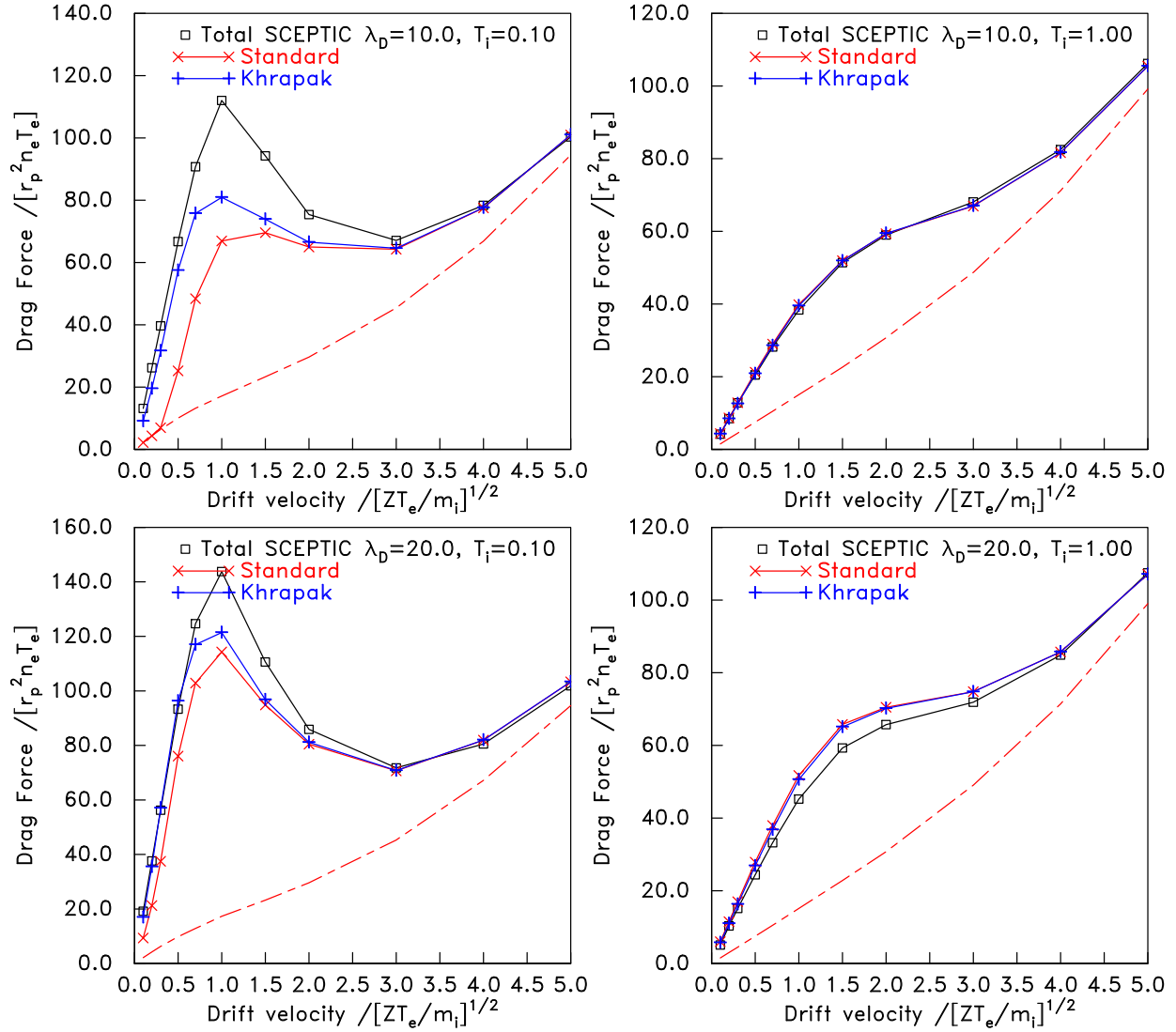
Figure 12: SCEPTIC calculations for \lambda_{De} = 10 and 20 , on a computational domain of radius 20 , and 40 times the probe radius; with T_i = 0.1 and 1.0 ZT_e .
