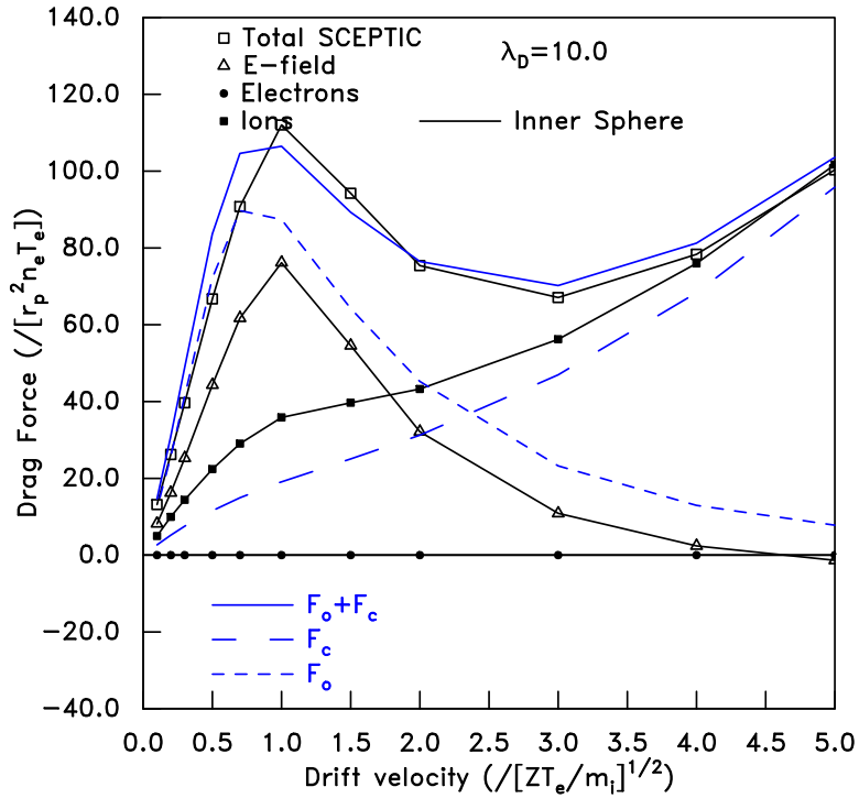
Figure 10: SCEPTIC calculations for \lambda_{De} = 10 , on a computational domain of radius 20, times the probe radius; with T_i = 0.1ZT_e . The contributions to the drag force at the inner surface do not correspond exactly to the theoretical orbit and collection components (shown dashed).
