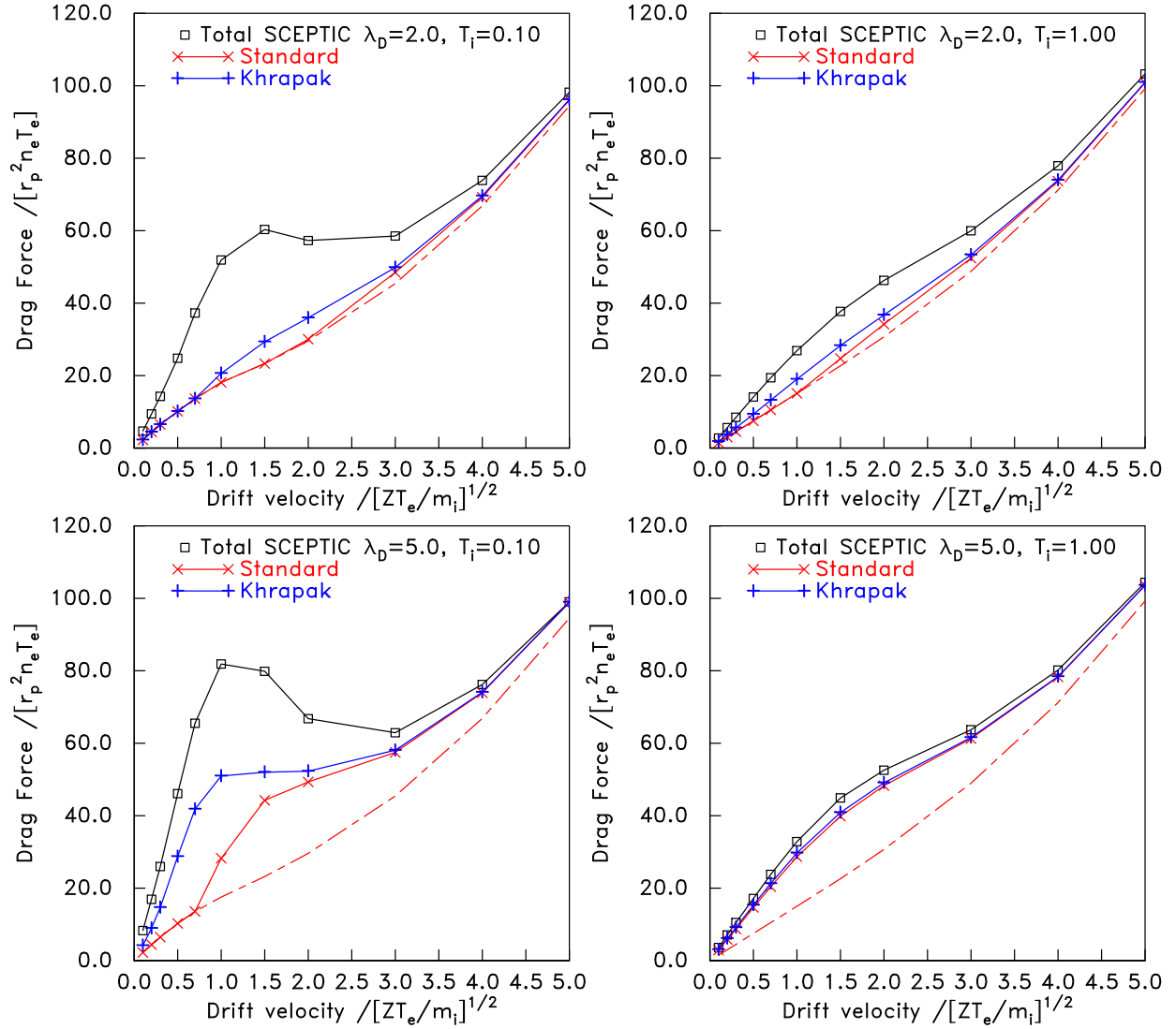
Figure 11: SCEPTIC calculations for \lambda_{De} = 2 and 5, on a computational domain of radius 10 and 20 respectively, times the probe radius; with T_i = 0.1 and 1.0 Z T_e .
