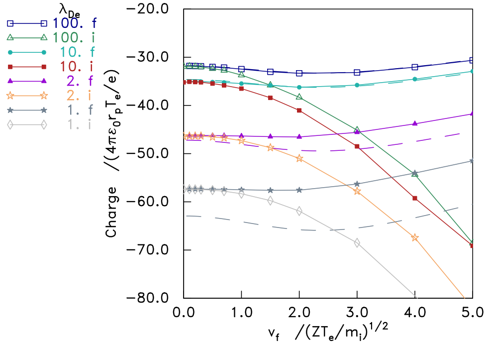
Figure 4: Charge as a function of drift velocity for an isolated sphere in a hydrogenic plasma ( m_i = 1837m_e , T_i = ZT_e ). A range of Debye lengths ( \lambda_{De} ) is plotted, and both floating (f) and insulating (i) spheres. Dashed lines show the linearized-capacitance analytic approximation.
