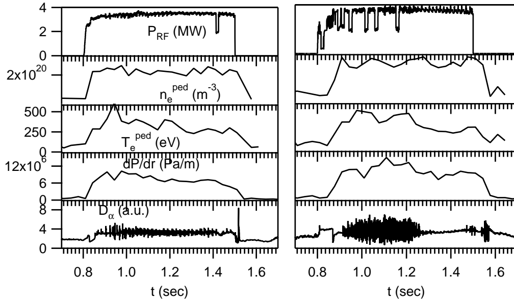
Fig.10 Traces of input power, pedestal density, temperature and pressure gradient and D_\alpha intensity for discharges with upper triangularity of 0.32 (a) and 0.45 (b). Increase of ELM amplitude and pedestal height and gradient is seen in higher delta discharge.
