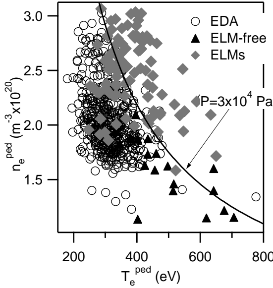
Fig. 7 Boundaries between EDA, ELM-free and ELM regimes in pedestal parameter space. Each point on the graph is a time point that could be identified as one of the three H mode types by fluctuation diagnostics. ELMs appear in the high pedestal pressure region.
