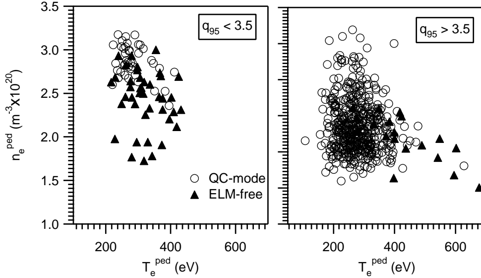
Fig. 5 Operational boundary of QC-mode in pedestal temperature ( T_e^{\text{ped}} ), density ( n_e^{\text{ped}} ) and edge q space
