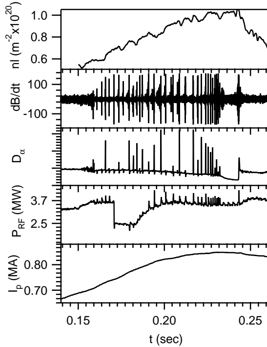
Fig. 11. ELMs driven by continuously rising plasma current in the RF induced H-mode in the initial phase of the discharge. Note changing ELM frequency as the current rise rate is changing and a transition to ELM-free H-mode when current rise stops.
