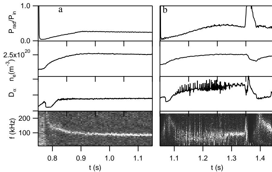
Fig.4 Magnetic fluctuation spectrum showing a QC mode and small ELMs together with divertor D_\alpha signal and traces of line integral density and total radiated power. In ELMy discharge the QC mode starts at \sim 1.04 s following L-H transition ( \sim 1.02 s) and brief ELM-free period. The mode is replaced by broadband fluctuations (ELMs) at \sim 1.05 s and reappears at \sim 1.23 s when edge temperature drops.
