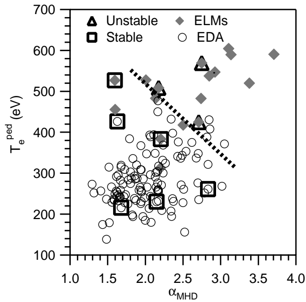
Fig. 9 Experimentally observed transition between EDA and ELMing regimes together with the results of ELITE stability analysis on a set of equilibria constructed for EDA and ELMing discharges
