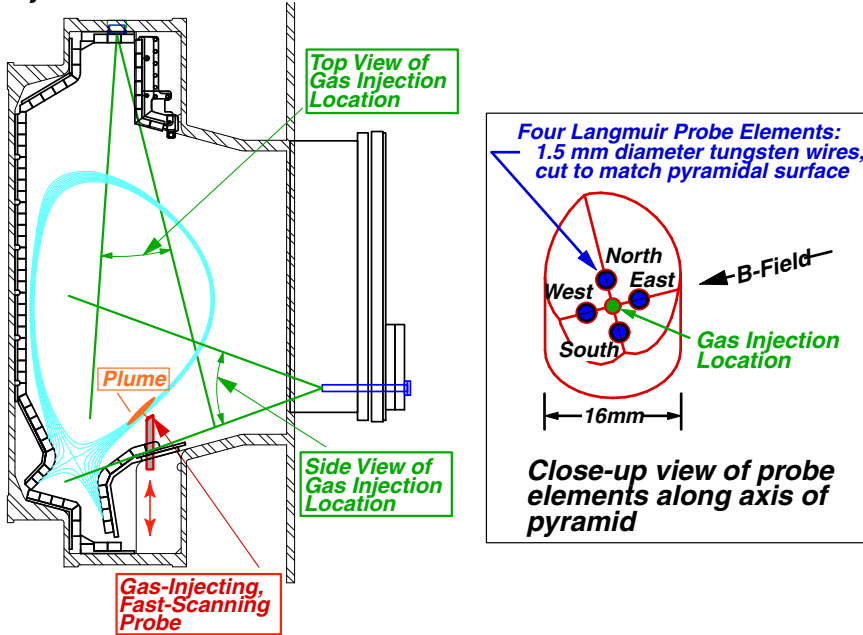
Fig. 1. (a) Cross-section of the Alcator C-Mod vacuum chamber with a typical diverted equilibrium. Gas is injected locally into the scrape-off layer at the end of stroke of a vertically-scanning probe. Impurity emission plumes are viewed from two near-perpendicular locations. (b) Close-up view of molybdenum probe head, indicating the location of the gas-injection capillary and the Langmuir probe elements used for density and temperature measurements and for providing estimates of the background flow.
