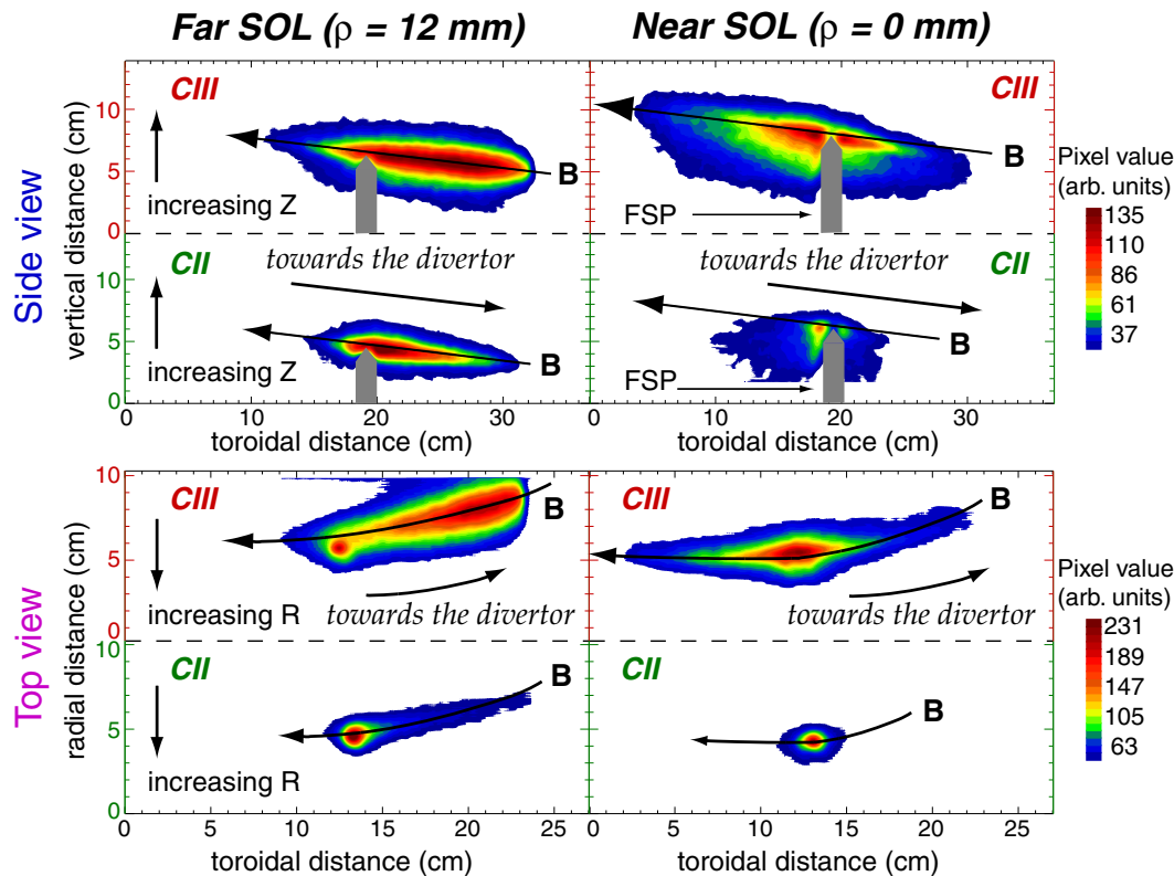
Fig. 2. Smoothed CII (514.1 nm) and CIII (465.0 nm) emission data from the side (SVC) and top (TVC) views. Both data were taken during Ohmic L-mode discharges. Data on the left was taken at a position in the far scrape-off layer, whereas data on the right was taken at the separatrix (indicated by \rho , which represents distance across flux surfaces mapped to the midplane). A schematic of the probe head is drawn in each figure to indicate its perturbation. An approximate local magnetic field direction is indicated to orient the emission.
