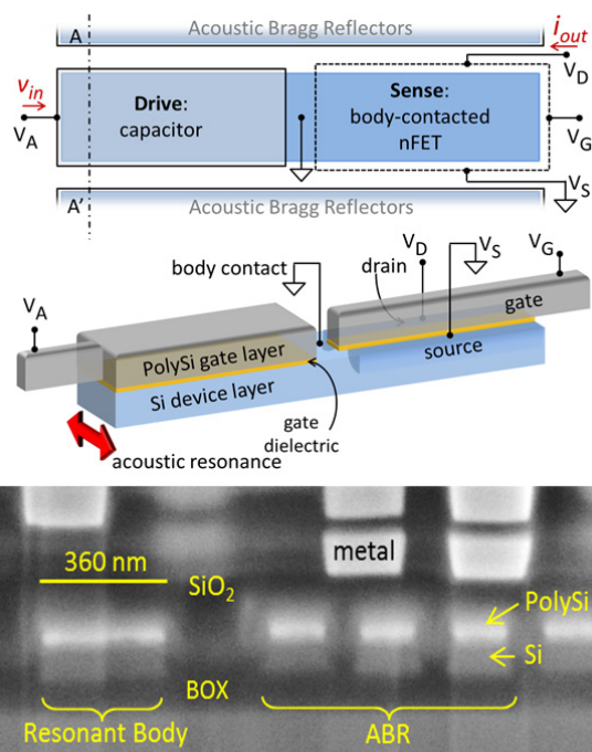
Fig. 1: Schematic and SEM of CMOS-MEMS Resonant Body Transistor. The resonant cavity is composed of the Si device layer and Poly gate layer, with Si Acoustic Bragg Reflectors (ABRs) adjacent to the resonant cavity.
