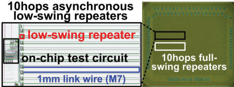
Fig. 4: Test chip die photograph in 45nm SOI CMOS.
