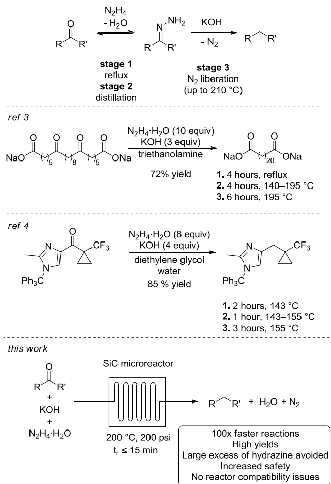
50 Scheme 1 Wolff-Kishner reductions in batch and flow.
