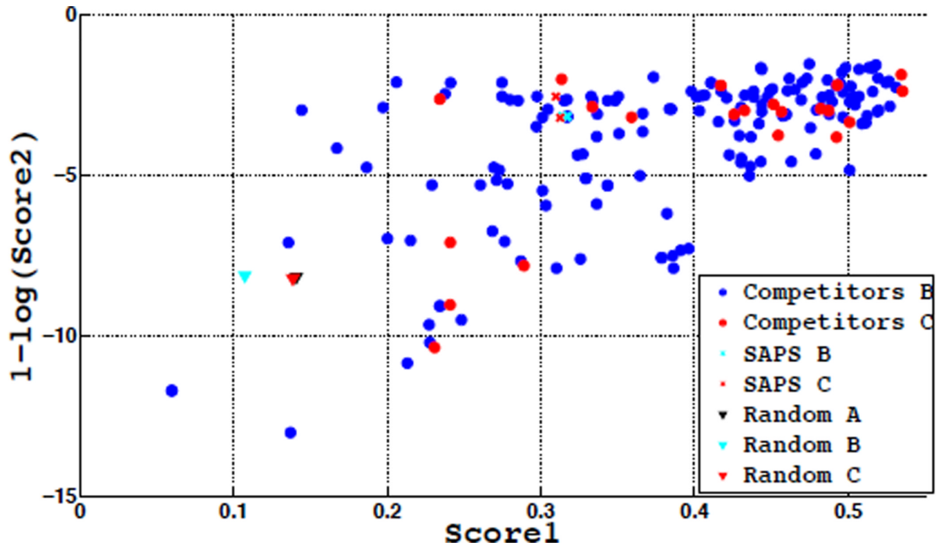
Figure 2. Scores for events 1 and event 2 on set B and C.
