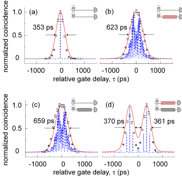
FIG. 2. (Color online) Temporal correlations of time-energy entangled photon pairs with (a) no dispersion; (b) signal photons propagating through no dispersion and idler photons propagating through normal dispersion; (c) signal photons propagating through no dispersion and idler photons propagating through anomalous dispersion; (d) signal and idler photons propagating through normal and anomalous dispersions, respectively. The insets show the configurations. Detuning: \delta/2\pi = 0.5\sigma_g/2\pi = 12 GHz. Open squares: experimental data; error bars: one standard deviation according to Poissonian statistics of the photon pairs; blue (gray) dashed lines: P(\tau) ; red (gray) solid lines: P_I(\tau) . Both experimental and numerical data are normalized to their maxima in each data set.
