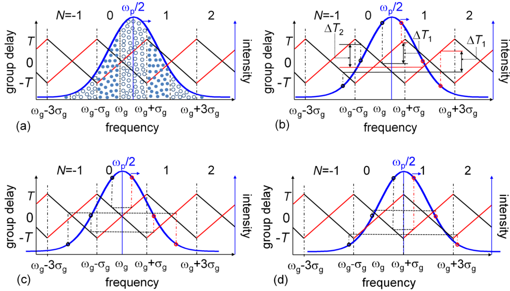
FIG. 4. (Color online) A graphic explanation of the double envelopes at general detunings ( \delta \neq 0 and \delta \neq \sigma_g ) and the single peaks at special detunings ( \delta = 0 and \delta = \sigma_g ). (a) At a general detuning ( \delta \neq 0 and \delta \neq \sigma_g ), the signal and idler photons experience different group delays resulting from the dispersive components. The group-delay differences have only two values: for the biphotons falling into the spectral region filled with open and filled circles, the group-delay differences are \Delta T_1 and \Delta T_2 , respectively, as shown in panel (b). These two group-delay differences correspond to two envelopes in the coincidence histogram. (c) At the detuning of \delta = 0 , the signal photon and its twin idler photon always experience the same group delay, corresponding to one peak at \tau = 0 in the coincidence histogram. (d) At the detuning of \delta = \sigma_g , the signal photon and its twin idler photon always experience the same group delay, corresponding to one peak at \tau = 0 in the coincidence histogram.
