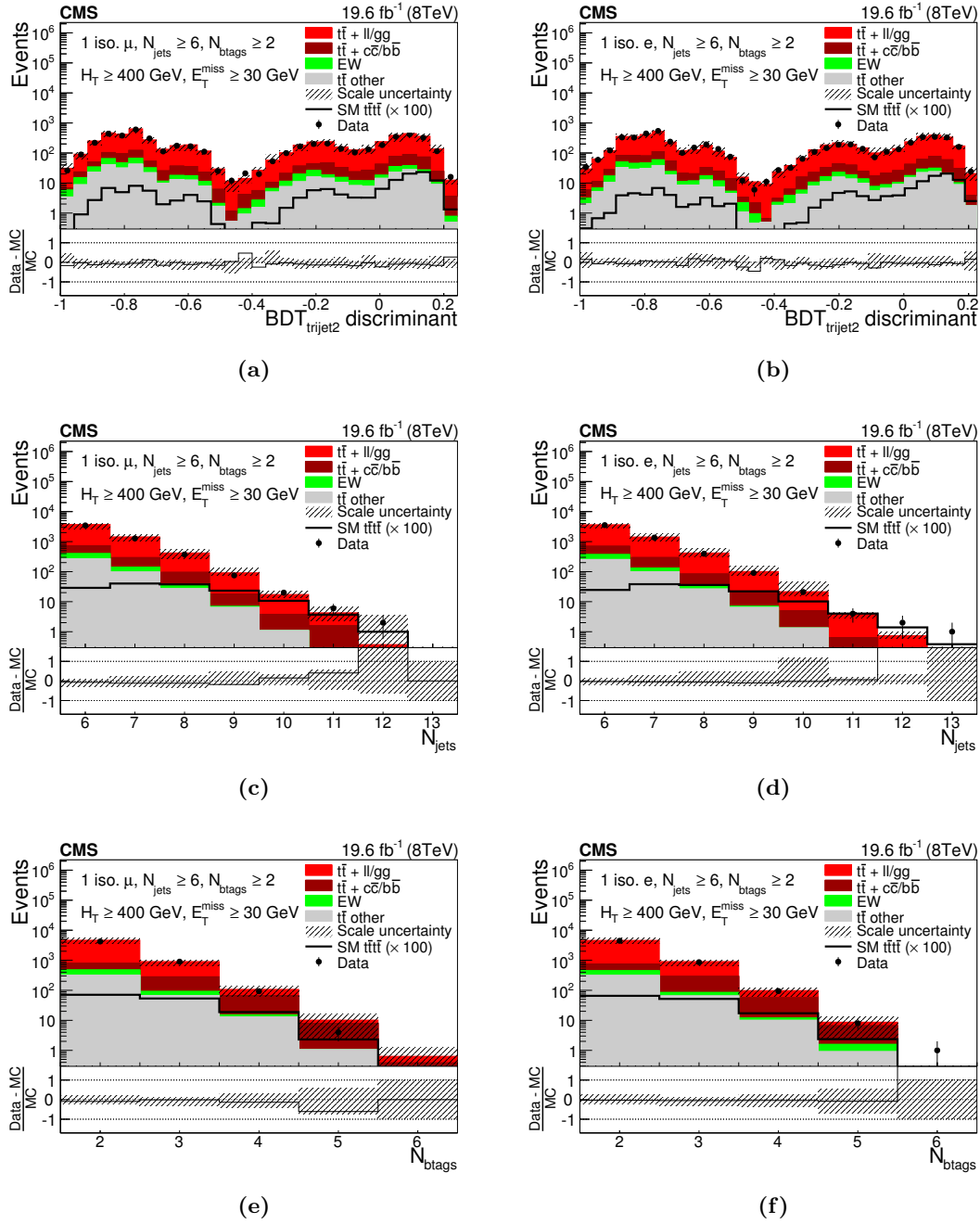
Figure 2. The distribution in the BDT_{\text{trijet2}} discriminant for the \mu + jets and e + jets channels in (a) and (b), respectively, and the same for N_{\text{jets}} in (c) and (d), and for N_{\text{btags}} in (e) and (f). The ratios plotted at the bottom of each panel reflect the percent differences between data and MC events. The hatched areas show the changes in the calculated predictions produced by factors of two and one half changes in the factorisation and renormalisation scales in the t\bar{t} simulation.
