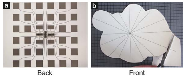
Figure 6: a) Backside of the fabricated multi-touch sensor featuring a grid of 6x6 electrodes. b) To guide the user, the front side features fine printed lines.
