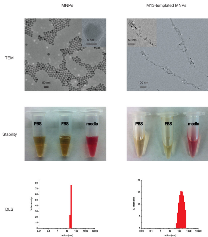
Figure 2. Material characterization of MNPs and M13-templated MNPs TEM (top row), stability (middle row), and dynamic light scattering (DLS) (bottom row) of synthesized and assembled iron oxide nanoparticles along the p8 major coat of M13 (left and right column, respectively). TEM of MNPs and M13-templated MNPs with higher resolution images in inset. For stability, samples were resuspended in PBS (left), serum (fetal bovine serum (FBS), middle) and tissue culture media (right). For DLS, MNPs were water-solubilized with NH 2 -PEG-DSPE (2000) and samples were run on a DynaPro Titan Light Scattering instrument at 10% power. Samples were run with n = 10.
