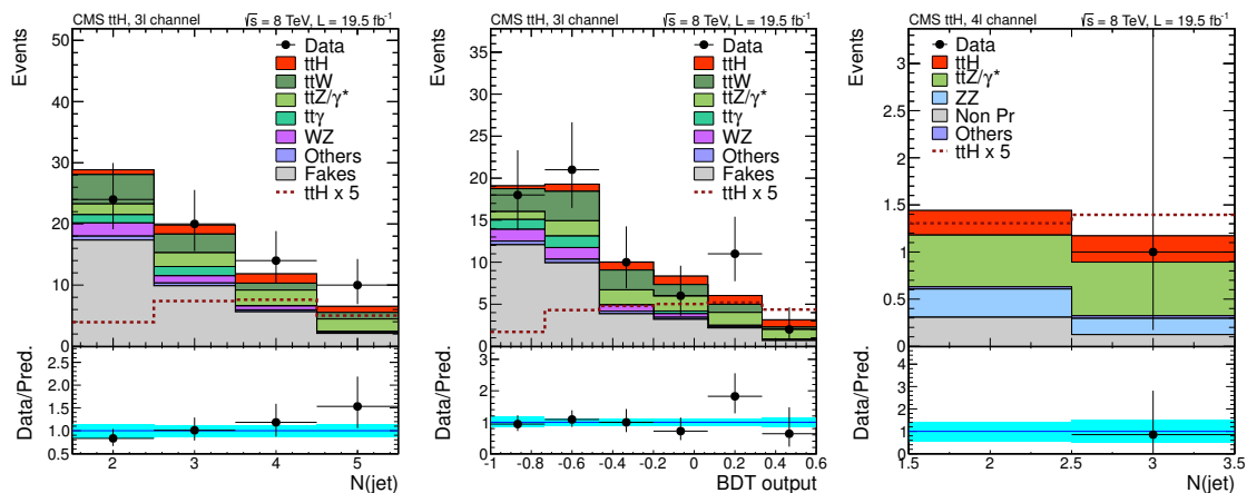
Figure 12. Distribution of the jet multiplicity (left) and BDT discriminant (center) for the triplepton search. Events with positive and negative charge are merged in these plots, but they are used separately in the signal extraction. The plot on the right shows the jet multiplicity for the four-lepton search. Signal and background normalizations are explained in the text. The b-tagged jets are included in the jet multiplicity.
