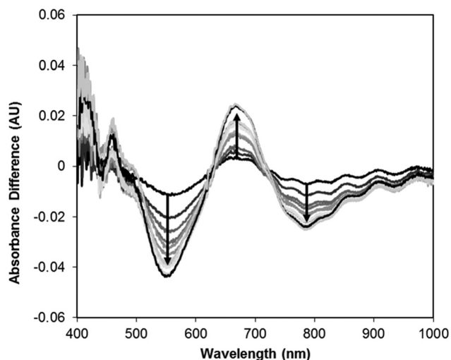
Fig. 14 Solid state difference absorption spectra of 5 relative to spectrum at 22 ^{\circ}\text{C} . Solid state spectra in KBr window at 0, -40 , -60 , -80 , -100 , -110 , -120 , -130 , -140 , -160 and -170 ^{\circ}\text{C} .
