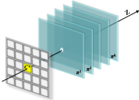
Figure 2. The 3D space is discretized using a set of K fronto-parallel planes, \{\pi^k\}_{k=1}^K , with respect to the central camera, C^0 .
