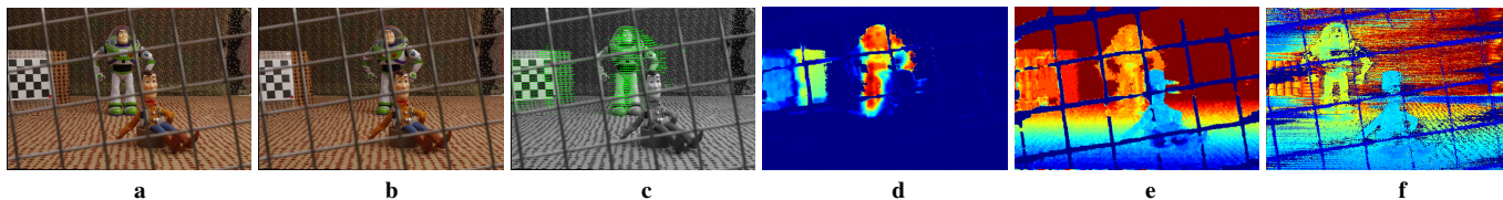
Figure 10. Real dataset (Toy Story): (a),(b) the reference view at time t and t + 1 , respectively; Buzz, as well as the check-board, moved; (c) the flow map of our optical flow; (d) the magnitude of our optical flow; (e) our depth map; (f) the estimated depth map using robust Voxel Coloring.
