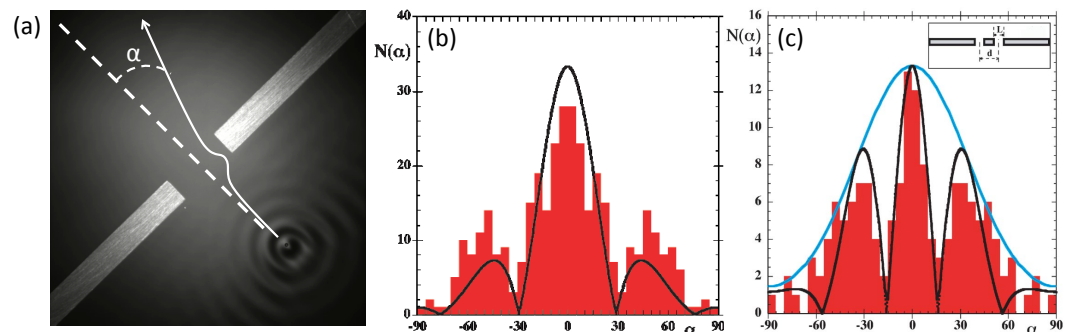
Figure 3: Single particle diffraction. a) A walker passes through a single slit. b) The histogram for the deflection angle \alpha from the single-slit experiments. b) The histogram for \alpha from the double-slit experiments. Reprinted from Couder & Fort (2006) with permission.
