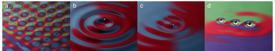
Figure 1: Image gallery. a) Faraday waves, just above threshold. b) A bouncing drop. c) A walker. d) A trio of bouncers. Photos courtesy of Dan Harris.
