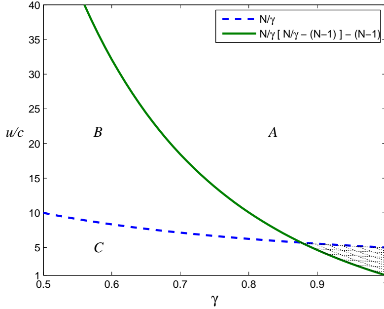
Figure 1 Conditions (13) and (15), with N = 5 .
