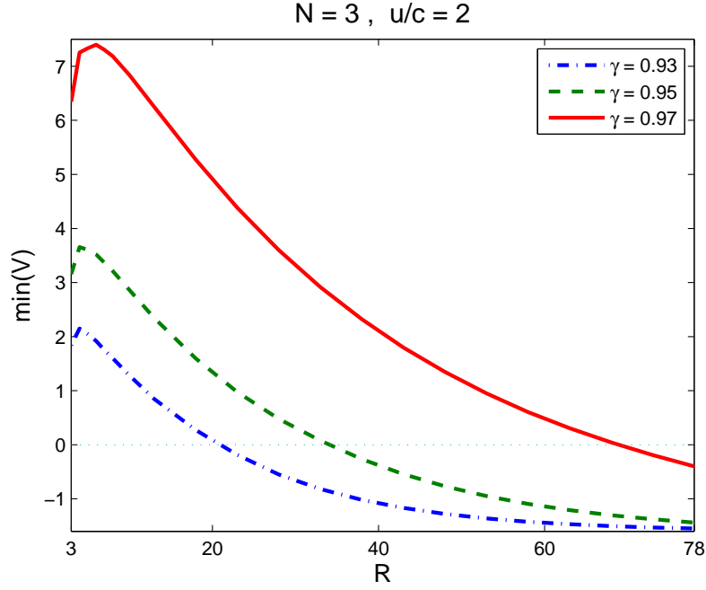
Figure 2 The non-monotone, unimodal structure of the value function in its minimum recurrent state.
