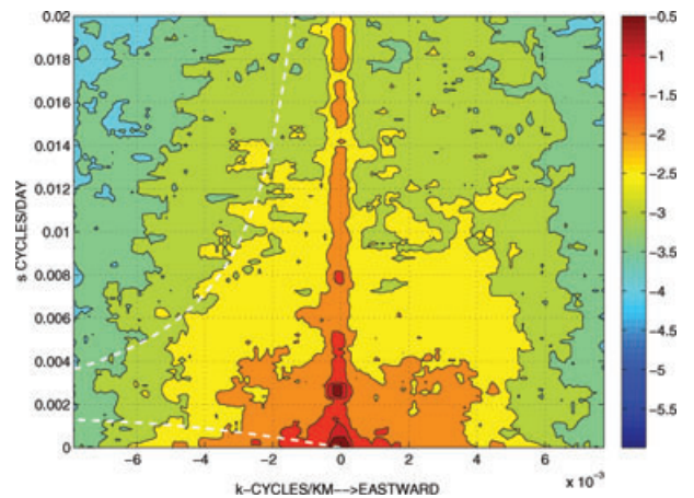
Fig. 3. \text{Log}_{10} of the zonal wavenumber–frequency spectral density estimate at 55°S, roughly the latitude of the Drake Passage, from 0° to 137°E. The non-dispersive line has vanished, and much energy is clustered around apparent long wavelengths, probably a direct wind-forcing response. Vanishing of the non-dispersive line occurs also at high northern latitudes (not shown). Note that there is some indication here of an excess of eastward-going phase velocities. In localized longitude bands at some latitudes, well-defined eastward going phase velocities can be seen in the data (C. Wortham, private communication, 2009).
