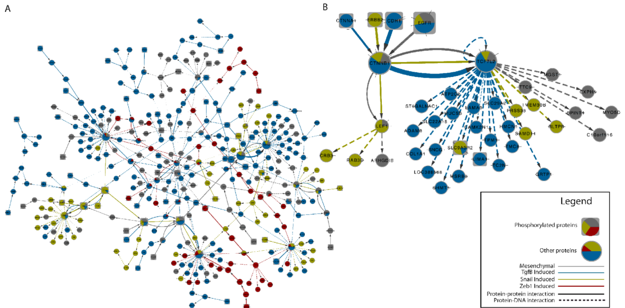
Figure 4. (A) Full EMT network annotated in a similar fashion to Figure 3. Phosphorylated proteins are represented by rectangles while non-phosphorylated proteins have grey borders. Pie charts represent flow distribution through nodes, while edge color represents the condition in which that edge was selected. (B) CTNNB1 and TCF7L2 and their interacting nodes.
