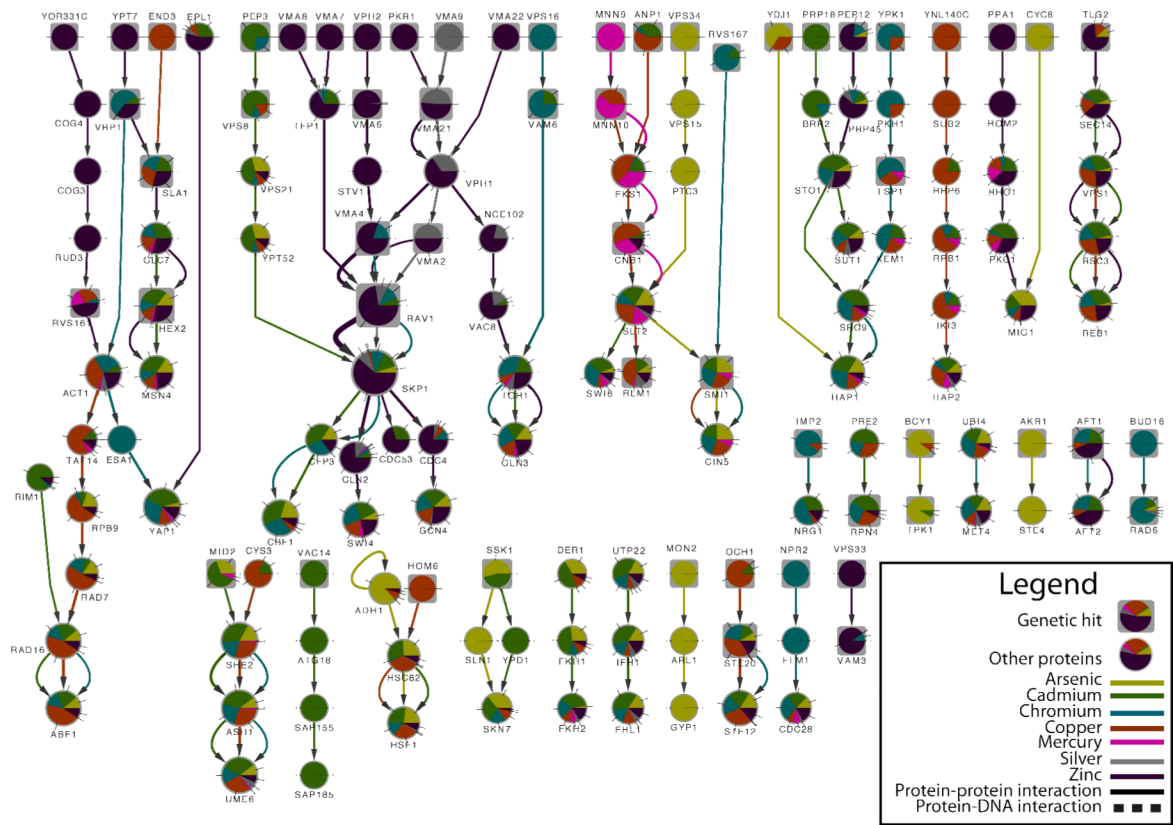
Figure 3. Subset of Yeast transition metal interactome with edge flow values greater than 0.005. Larger node size indicates more flow, while color indicates conditions in which that node/edge is determined to be active. The direction of edges represents flow from genetic hits (rectangles) to mRNA nodes and the color of the edges represents the commodity that was selected to use that edge. Pie charts correspond to fraction of flow for each commodity passing through the node. Graph generated and filtered by Cytoscape 28
