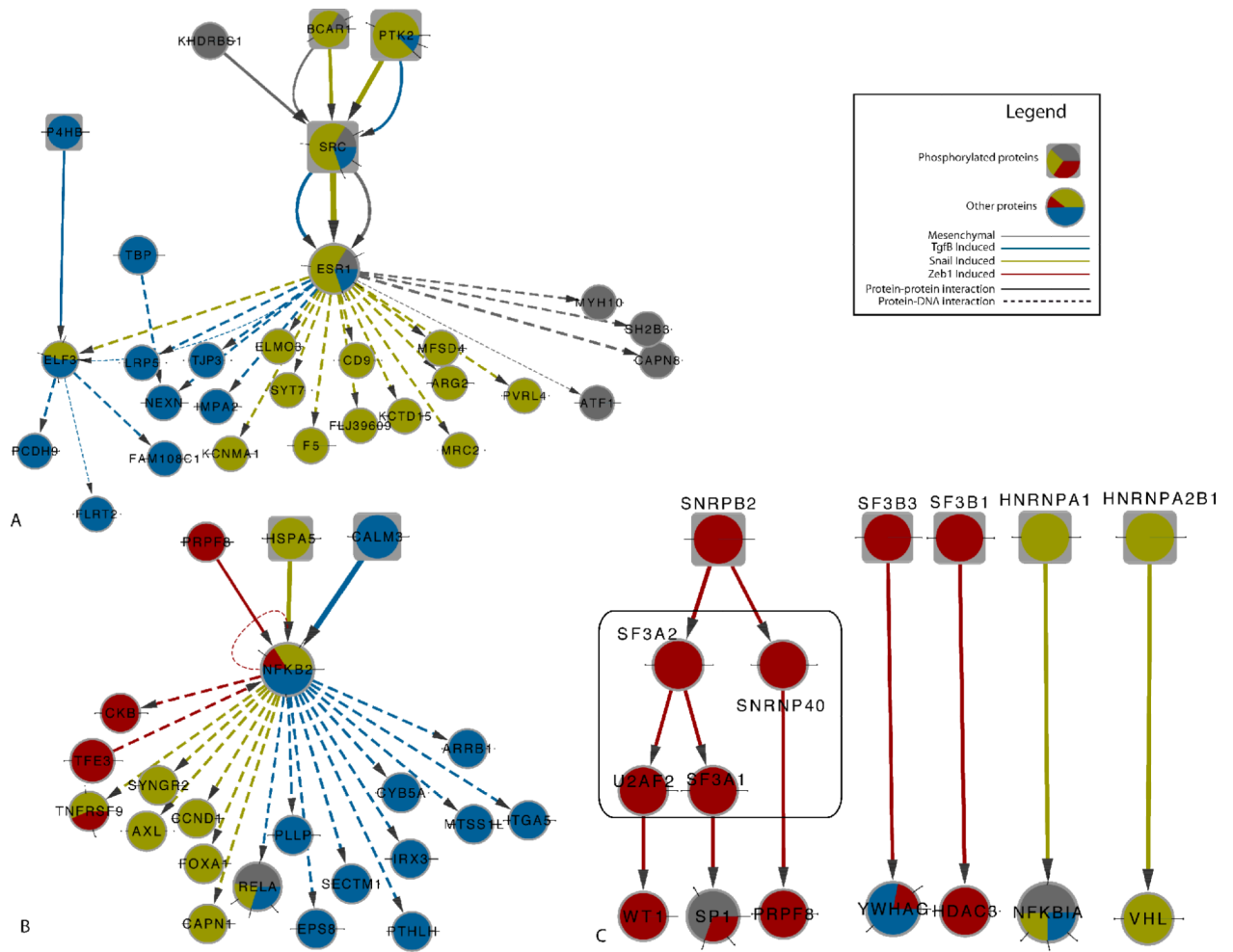
Figure 5. (A) Role of ESR1 in Snail and TGFβ pathways (B) NFKB2 activity in induced models only (C) Spliceosome-related proteins (according to KEGG) and their interacting partners identified by SAMNet in two induced models. Differentially phosphorylated proteins are represented by rectangles while those inferred by SAMNet are encircled in the black square.
