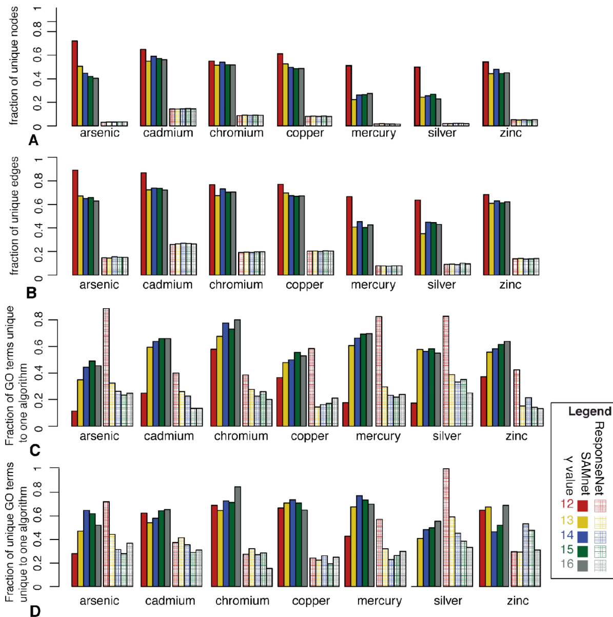
Figure 2. Comparison of SAMNet and ResponseNet. Fraction of unique (A) nodes and (B) edges in each commodity of SAMNet for the various values of \gamma compared to the original ResponseNet networks on each independent condition. Fraction of (C) all and (D) unique (to a specific condition) GO terms identified by SAMNet (per commodity) and ResponseNet (on corresponding condition).
