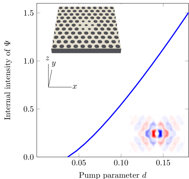
FIG. 8. (Color online) 3D calculation of a lasing mode created by a “defect” in a photonic-crystal slab [13]: a period- a hexagonal lattice of air holes (with a = 1 \text{ mm} and radius 0.3 \text{ mm} ) in a dielectric medium with index n = \sqrt{\varepsilon_c} = 3.4 with a cavity formed by seven holes of radius 0.2 \text{ mm} in which a doubly-degenerate mode is confined by a photonic bandgap (one of these degenerate modes is selected by symmetry, see text). The gain has \gamma_{\perp} = 2.0 \text{ mm}^{-1} , k_a = 1.5 \text{ mm}^{-1} , and non-uniform pump D_0(\mathbf{x}, d) = f(\mathbf{x})d , where the pump profile f(\mathbf{x}) = 1 in the hexagonal region of height 2 \text{ mm} in the y -direction, and f(\mathbf{x}) = 0 outside that region and in all air holes. The slab has a finite thickness 0.5 \text{ mm} with air above and below into which the mode can radiate (terminated by PML absorbers). The inset shows magnetic field H_z ( \sim \partial_x E_y - \partial_y E_x ) of the TE-like mode at the z = 0 plane.
