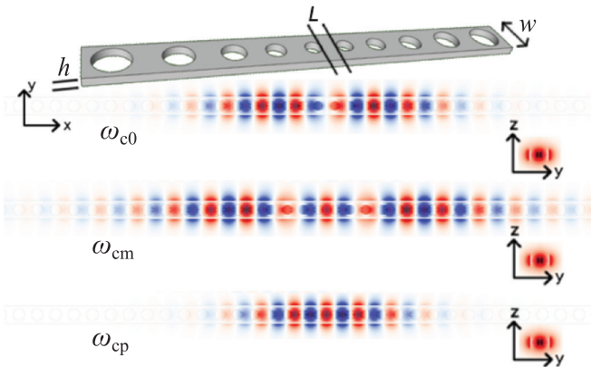
FIG. 2. (Color online) Schematic of 3D triply resonant cavity design involving a PhC nanobeam of refractive index n = 3.4 , width w = a , and height h = 0.51a , and linearly tapered air holes, as described in the text. The central cavity length L \approx 0.4a and number of taper segments are chosen so as to fine-tune the relative frequency spacing and lifetimes of the modes. Also shown are the E_y electric-field components of three TE-like modes with fundamental TE00 transverse profiles, and with frequencies \omega_{c0} = 0.2848(\frac{2\pi c}{a}) , \omega_{cm} = 0.2801(\frac{2\pi c}{a}) , and \omega_{cp} = 0.2895(\frac{2\pi c}{a}) . Radiation lifetimes are found to be Q_0^{\text{rad}} = 10^6 , Q_m^{\text{rad}} = 3 \times 10^4 , and Q_p^{\text{rad}} = 2 \times 10^4 .
