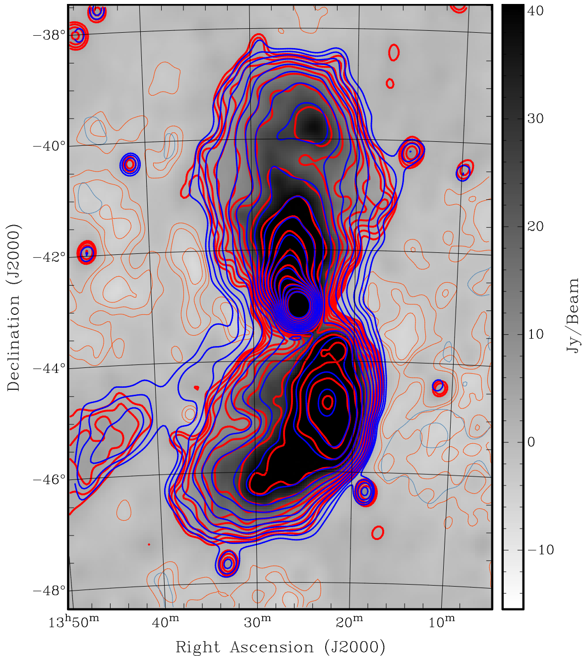
Figure 6. Cen A at 118 MHz (greyscale and red contours) overlaid with Parkes 1.4 GHz contours in blue, smoothed to the same angular resolution of 25 arcmin. Positive contours are bold and start at 2.5 Jy/beam for 118 MHz and 0.50 Jy/beam for 1.4 GHz, incrementing in a geometric progression of \sqrt{2} . Negative contours (thinner and lighter shade) start at -2.5 Jy/beam for 118 MHz and -0.50 Jy/beam for 1.4 GHz and decrement in a geometric progression of \sqrt{2} .
