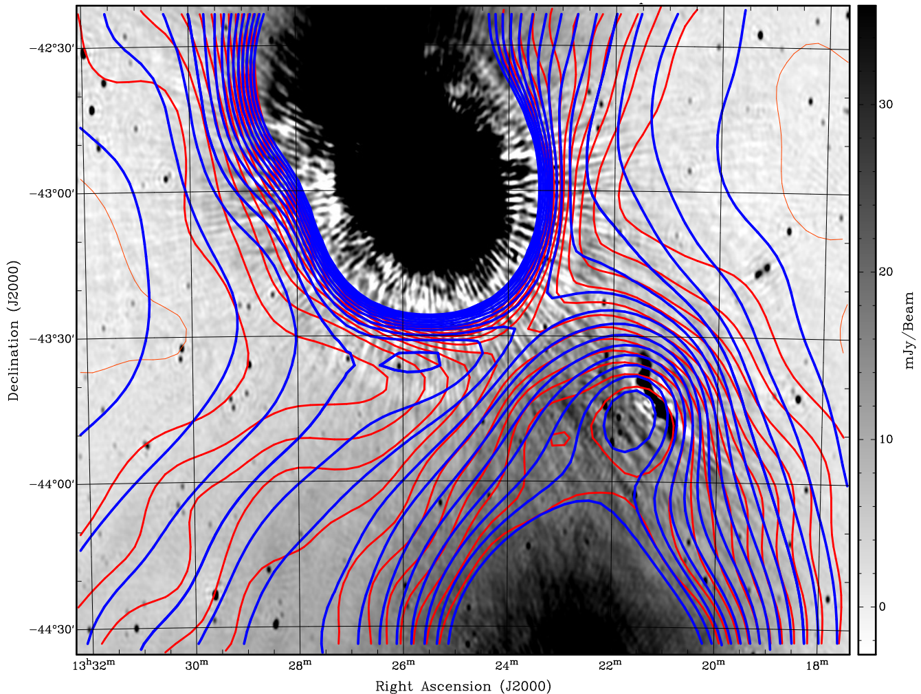
Figure 11. High resolution 1.4 GHz Parkes+ATCA map (Feain et al. 2011) in greyscale, overlaid with the 1.4 GHz Parkes contours (O’Sullivan et al. 2013) in blue and the MWA 118 MHz contours in red. Positive 118 MHz MWA contours are from 3 Jy/beam incrementing in steps of 5 Jy/beam and 1.4 GHz Parkes contours are from 1 Jy/beam incrementing in steps of 1 Jy/beam. There is one negative contour visible, which is the -3 Jy/beam level of the 118 MHz map, shown as a thinner, lighter red line. There is a peak at 13^{\text{h}}23^{\text{m}}, -43^{\circ}51' in the 118 MHz map that is not visible in the 1.4 GHz images and does not coincide with any background sources visible at 1.4 GHz. The bright background source MRC 1318-434B, at 13^{\text{h}}21^{\text{m}}18^{\text{s}}, -43^{\circ}41'15'' , extends approximately 20 arcmin and is coincidentally aligned with the position angle of the inner lobes of Cen A.
