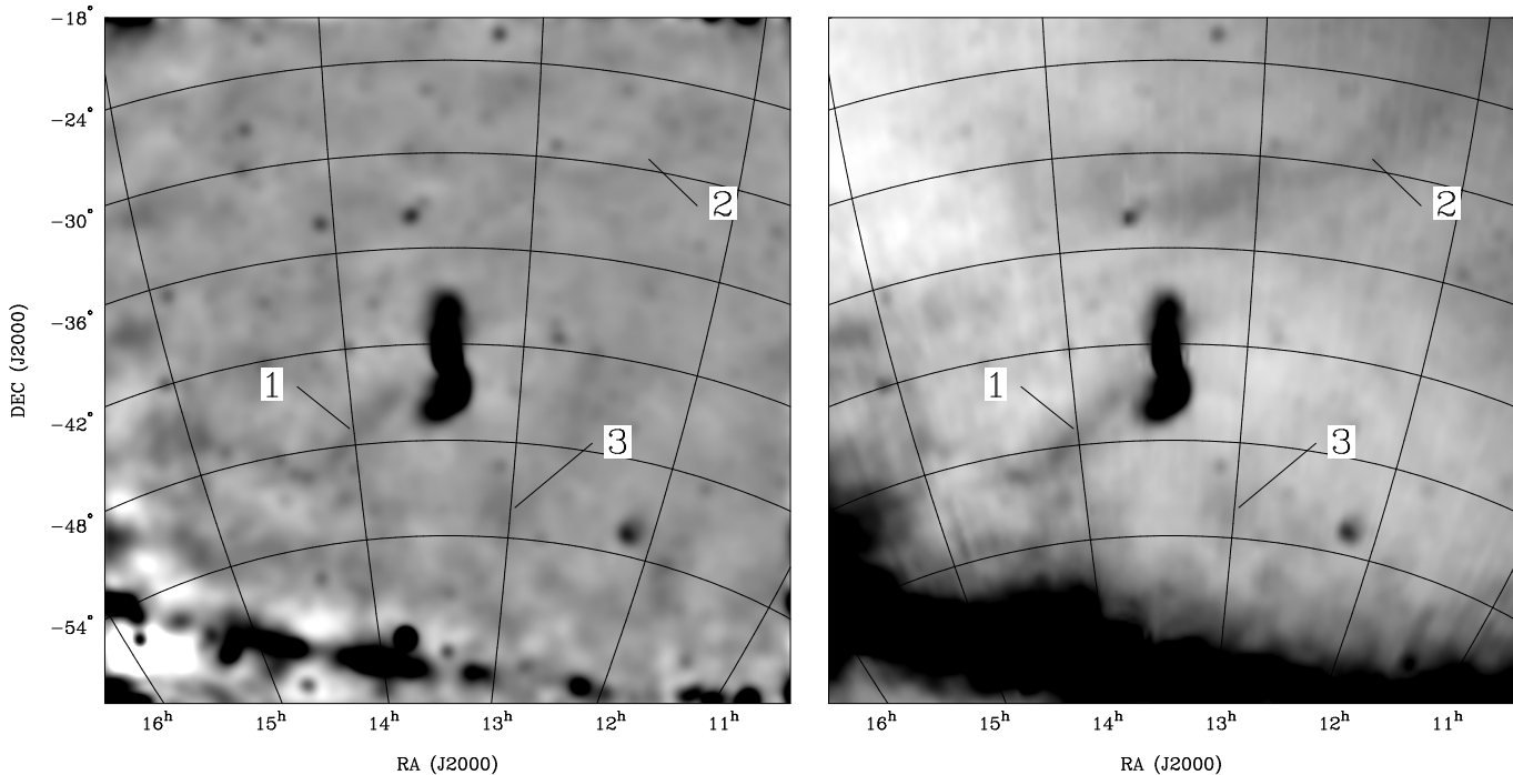
Figure 5. Comparison between the MWA 118 MHz image (left) and Haslam et al. (1982) 408 MHz image (right), both smoothed to the same angular resolution of 0.85^\circ . A linear brightness gradient has been subtracted from the Haslam et al. (1982) map to make the smaller-scale structures clearer. The faint diffuse structure on scales less than 12^\circ matches well by eye. Labels 1 to 3 indicate large-scale foreground features clearly present in both maps.
