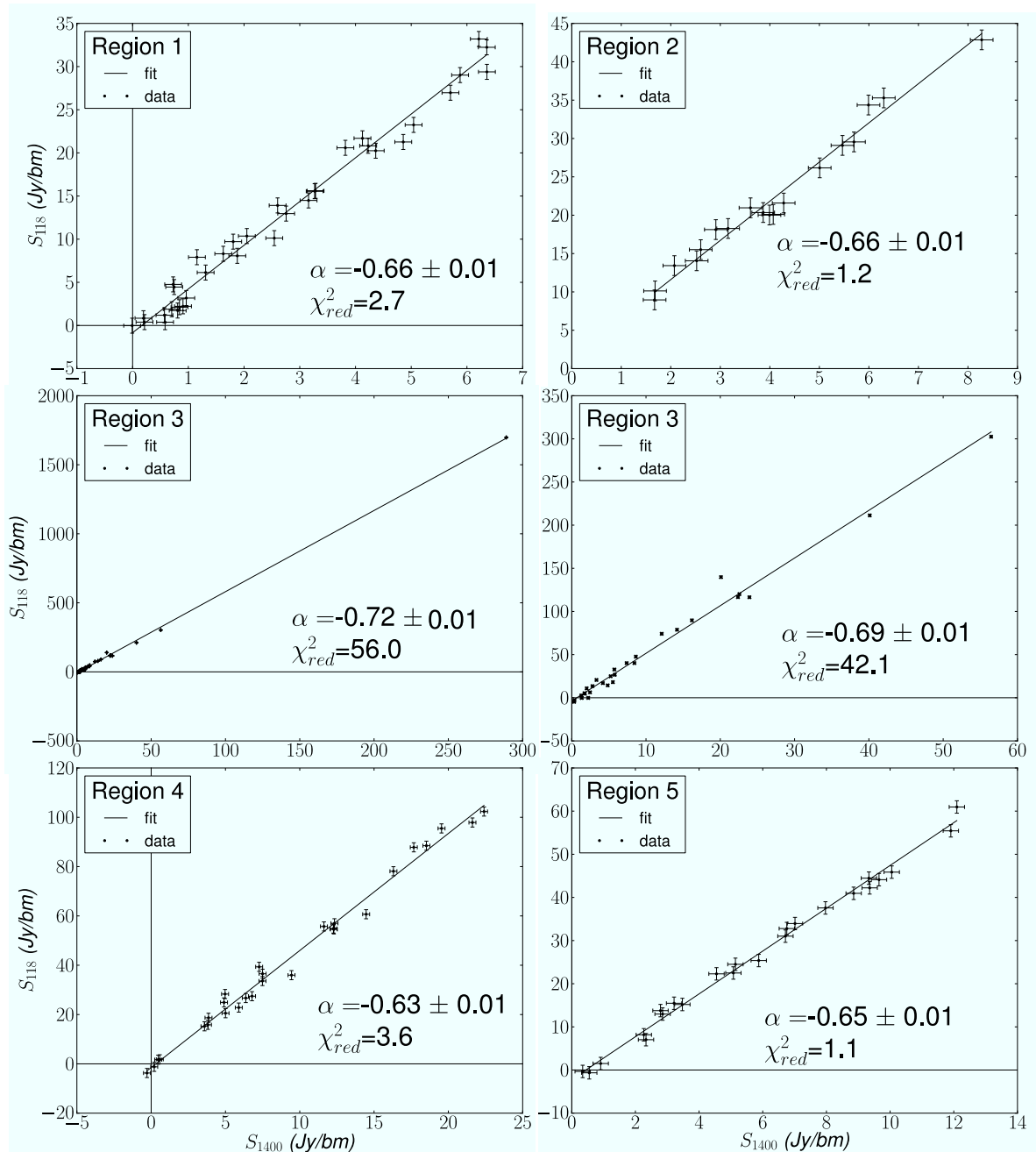
Figure 8. T-T plots for the five regions of the giant lobes of Cen A and the computed spectral indices between 118 MHz and 1400 MHz, including the \chi_{red}^2 values for each region as defined in Fig. 7. The centre row contains two plots for region 3; on the left all pixels have been included, and on the right the bright central pixel has been excluded to remove the influence of the inner lobes. The uncertainties in the spectral indices displayed are derived from the uncertainty in the slope of the line of best fit and represent random errors only. See text for the inclusion of systematic errors due to global flux scale uncertainties.
