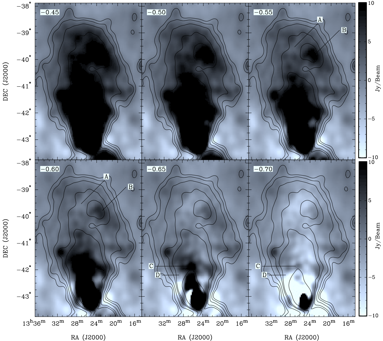
Figure 9. A subset of the spectral tomography images of the northern lobe between 118 MHz and 1.4 GHz with trial spectral indices as indicated in the top-left corner of each sub-image. Greyscale is from -10 to 10 Jy/beam. Overlaid are contours from the 118 MHz image at 2.5, 5, 10, 20, 28.3 and 113 Jy/beam. The feature labelled A has a significantly flatter spectral index than that labelled B. Similarly, there is a change in spectral index between the flatter region labelled D and the steeper feature labelled C.
