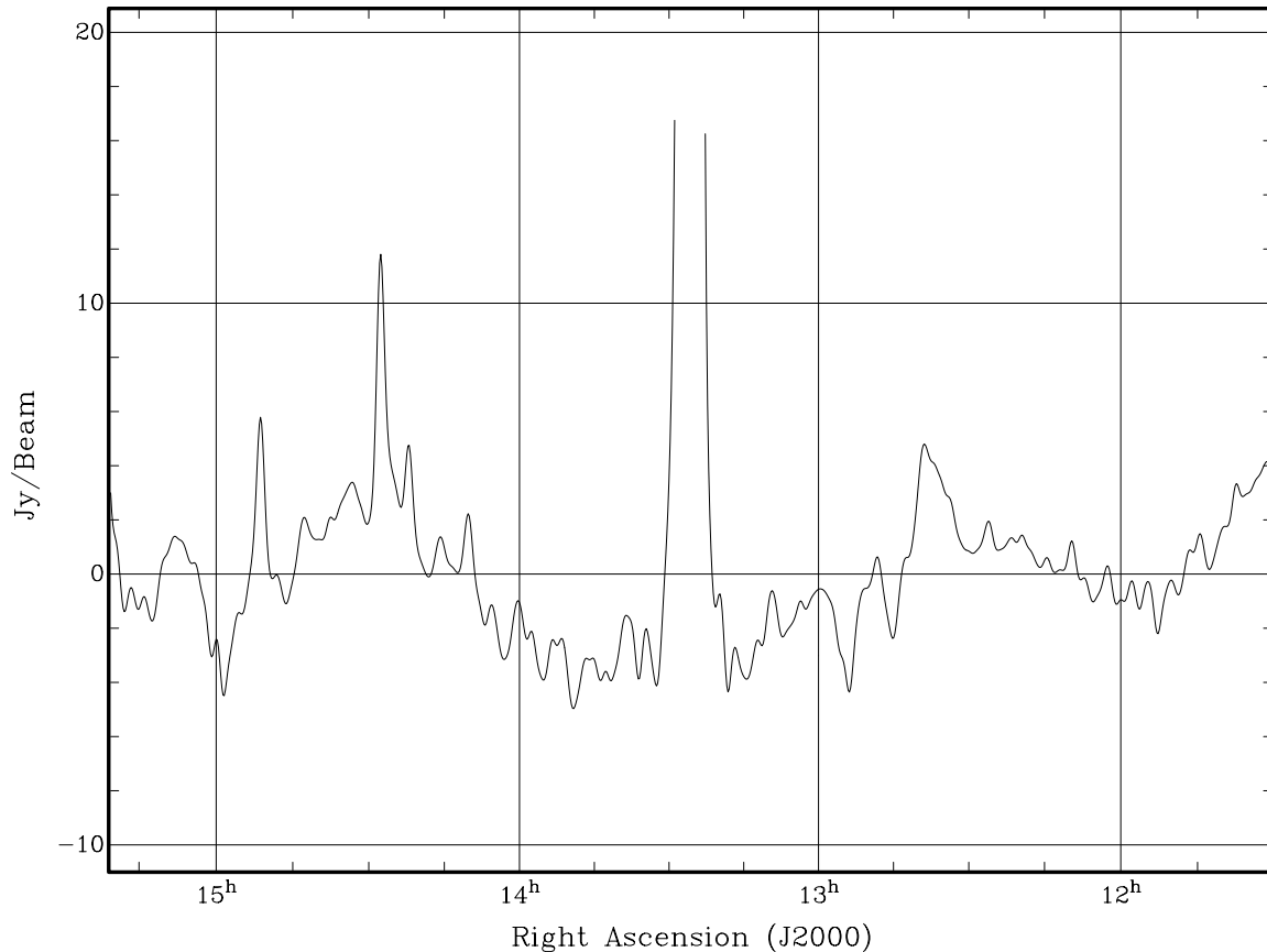
Figure 4. Profile through the centre of the MWA 118 MHz image of Cen A (see Fig. 3) along a constant declination of (J2000) -43^{\circ}01'9'' , showing the negative bowl surrounding the core of Cen A in the image.
