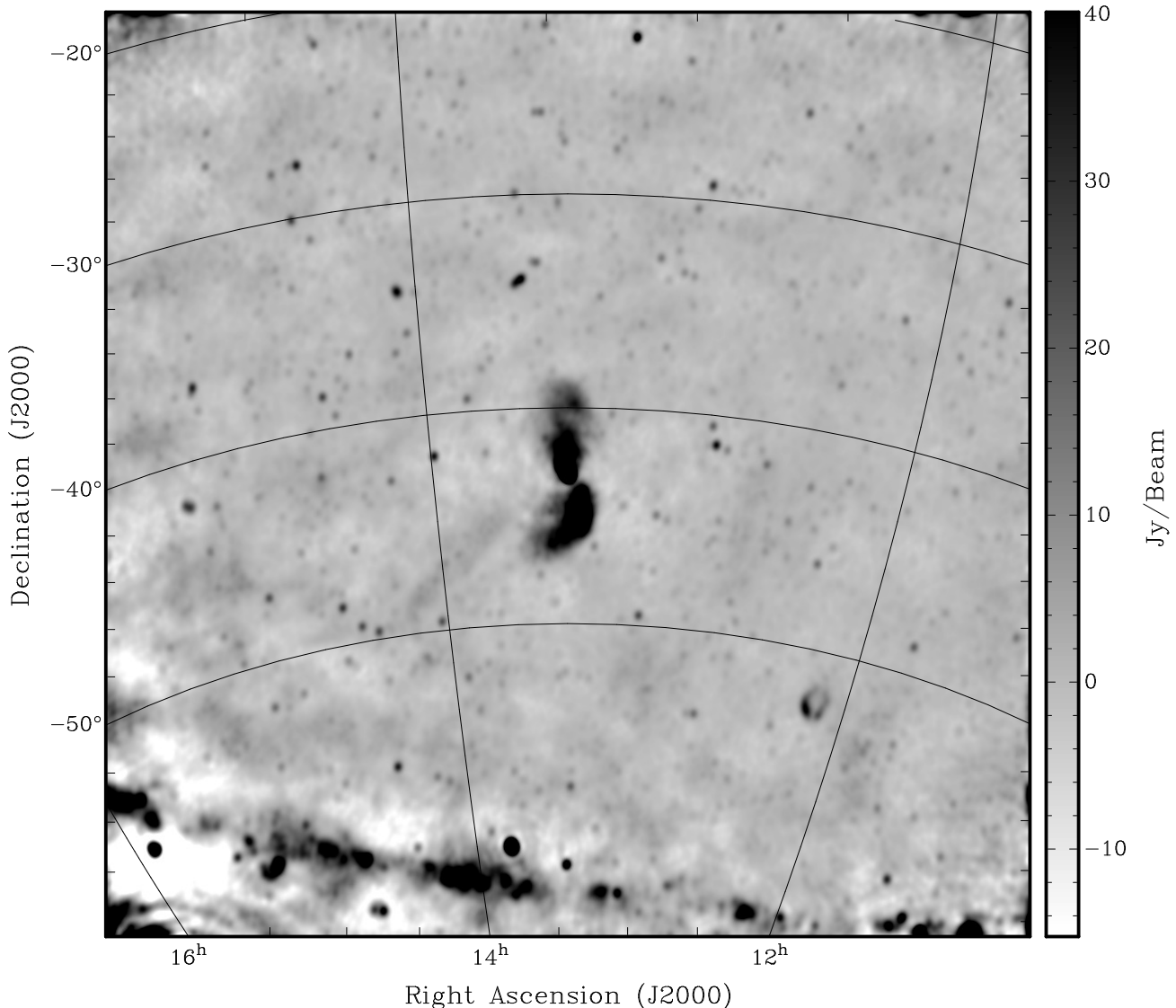
Figure 3. Cen A and surrounding field at 118 MHz with the Murchison Widefield Array 32-Tile prototype. The image is shown on a linear scale between -15 and +40 Jy/beam. It has an angular resolution of 25 arcmin and an rms noise of approximately 0.5 Jy/beam in ‘empty’ regions of the map.
