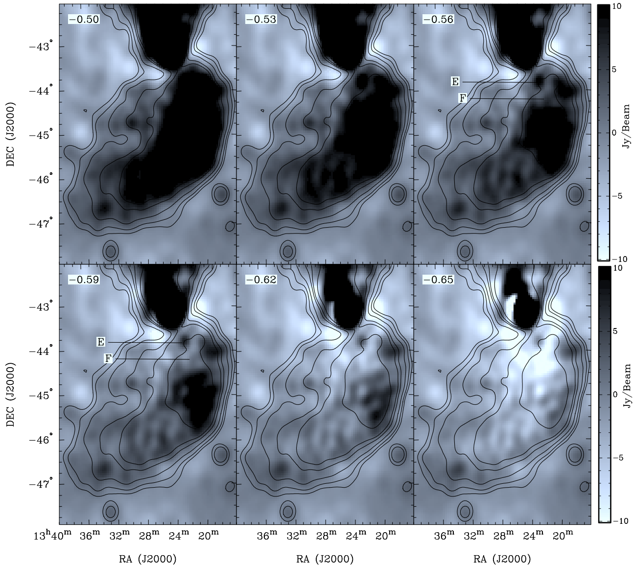
Figure 10. As for Fig. 9, but for the southern lobe with contours from the 118 MHz image at 2.5, 5, 10, 20, 28.3 and 56.5 Jy/beam. The feature labelled E has a significantly steeper spectral index than that labelled F.
