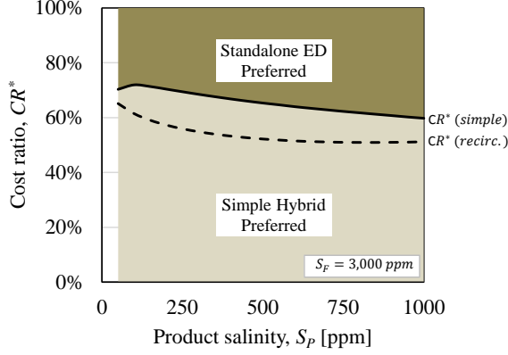
Figure 6: Dependence of the optimality of hybrid systems upon the cost ratio and the product salinity.
