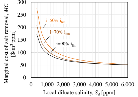
Figure 8: Illustration of the sensitivity of the marginal cost of salt removal to cell pair voltage.
