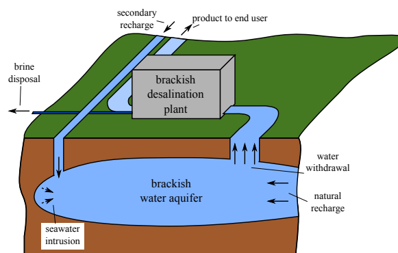
Figure 1: The supply of freshwater and mitigation of seawater intrusion with brackish desalination and secondary recharge. Based on an aquifer management system proposed by Koussis et al. [4].
