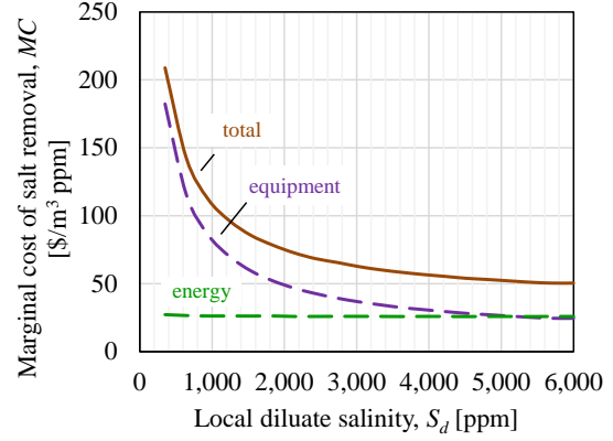
(b) Marginal cost of salt removal
