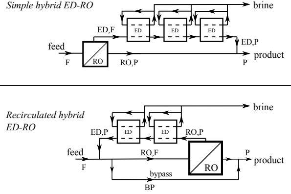
Figure E.9: Simple and recirculated hybrid systems with streams labelled
