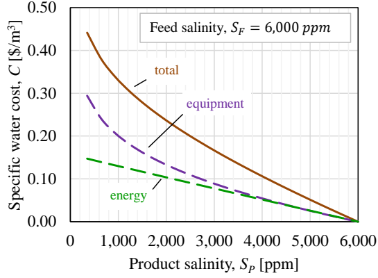
(a) Specific water cost
