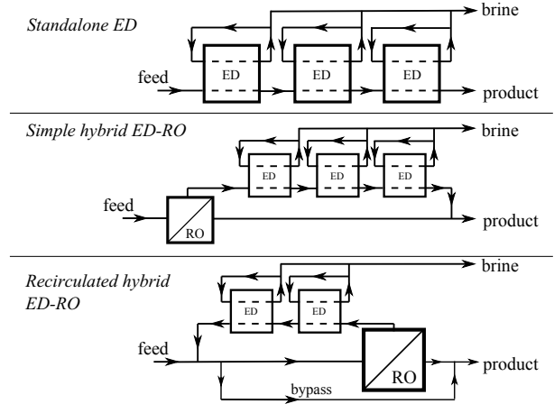
Figure 3: Standalone and hybrid ED configurations. The relative size of electrodesalination (ED) and reverse osmosis (RO) units is intended to illustrate the relative quantities of membrane area required in each, assuming the final product flow rate from all systems is the same.
