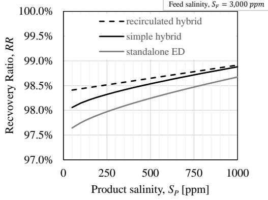
Figure F.10: System recovery ratios
