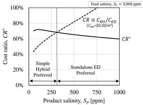
Figure 7: The ratio of water costs from single stage RO rise relative to ED as product salinity increases. At low product salinities a hybrid system can therefore be justified as the cost ratio falls below the critical cost ratio CR^* while at higher product salinities a standalone ED system is preferable.
