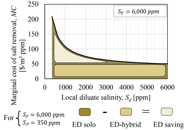
Figure 5: Cost savings can be achieved by shifting electro dialysis salt removal to higher salinity.
