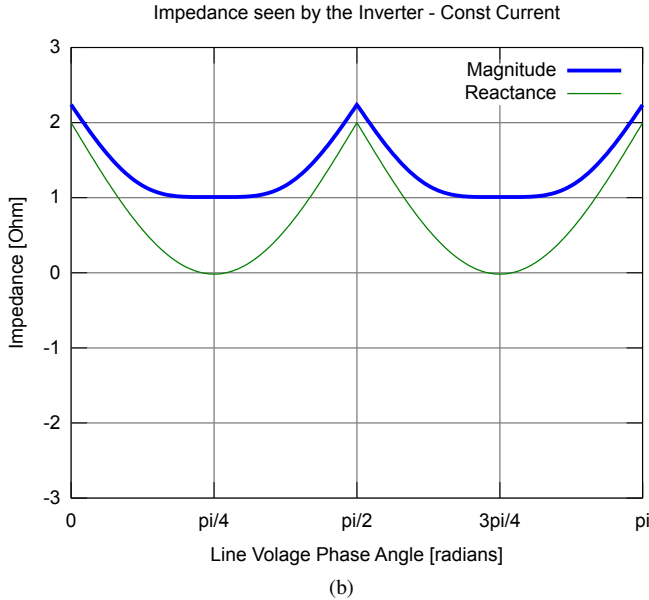
Fig. 12. The normalized load impedance, at the switching frequency, presented to the full-bridge inverter by (a) the buffer-block, and cycloconverter stages, and (b) including the series-resonant tank. Without the inductance of the resonant tank, the reactance presented to the inverter prevents zero-voltage switching.
