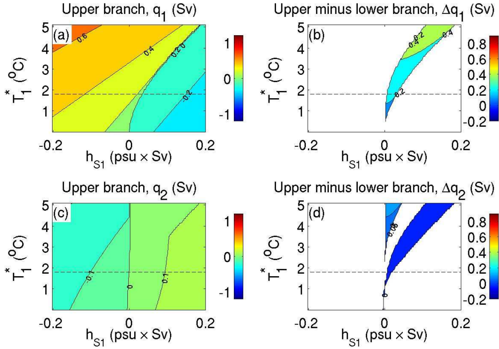
Figure 5: (a) Flux, q_1 (in Sv) between the Adriatic and Ionian boxes as a function of surface Adriatic-Ionian salinity flux, h_{s_1} and the Adriatic-Ionian apparent temperature T_1^* . The largest of two possible value of q_1 is depicted. (b) Same as (a) for the flux difference between the larger and smaller q_1 ; only the region of bi-stability is plotted. (c) Same as (a) for Aegean-Ionian flux. (d) Same as (b) for the Aegean-Ionian flux. Note the small values in panels (c),(d), indicating that the Adriatic-Ionian interaction is almost decoupled from the Aegean-Ionian interaction. The horizontal dashed line indicates the Adriatic-Ionian apparent temperature, T_1^* , given in Table 1.
